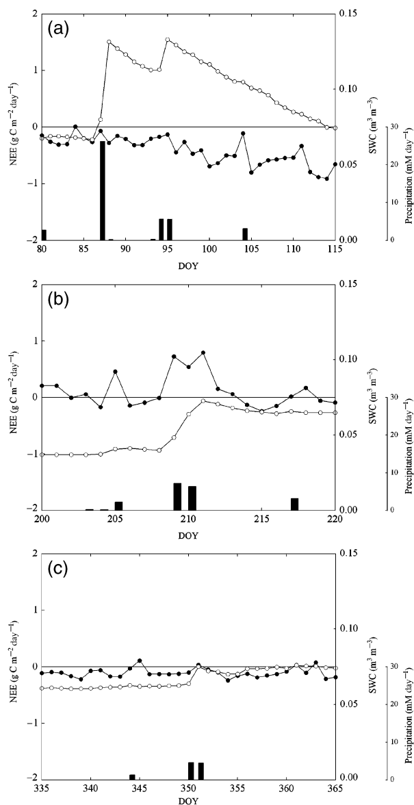
Fig. 8 Selected time series of daily sums of net ecosystem \text{CO}_2 exchange (NEE, filled symbols), daily precipitation (black bars) and daily average soil water content (SWC, open symbols) for illustrating precipitation effects on NEE. Time periods represent: March/April 2006 (a), July/August 2005 (b) and December 2006 (c).
