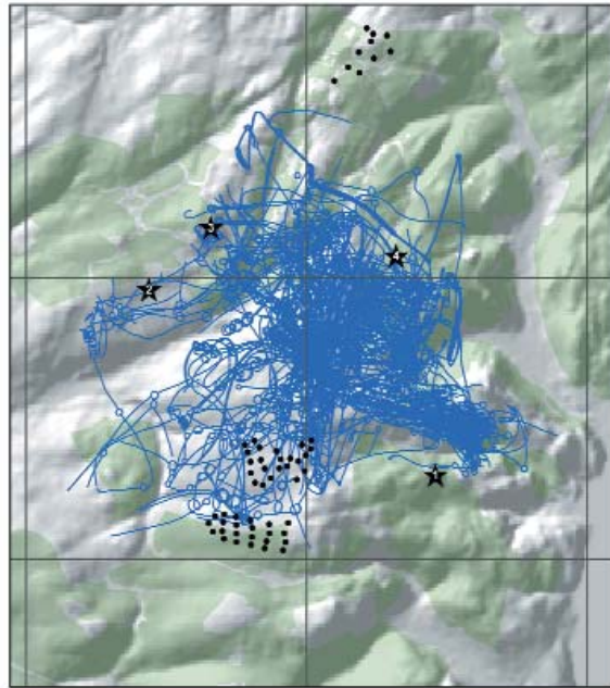
Figure 3 Flight lines (left, n=811) of resident Golden Eagles (male and female). Grid (1 km 2 ) colour shows relative use by eagles (dark red=heavy use, light pink=light use).
