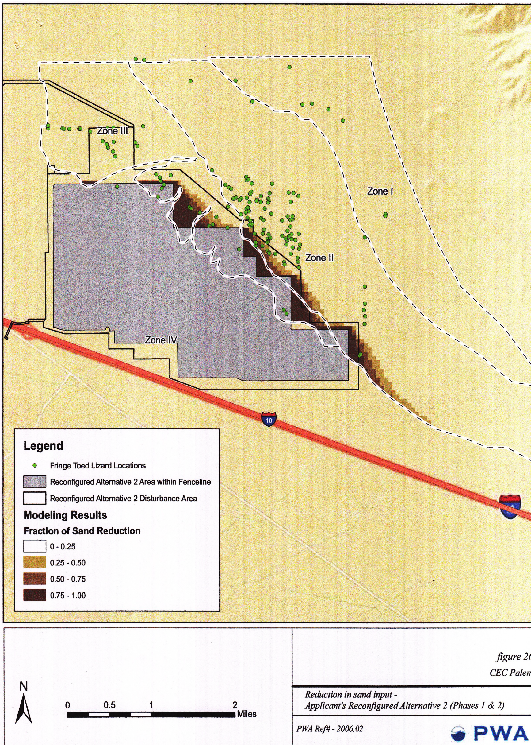
Figure 13. Diagram showing the calculated fraction of sand reduction determined by the Collison model, using the Applicant's Reconfigured Alternative 2 (Phases 1 and 2) facility configuration. The Collison model predicts 144 acres of indirect impacts and 680 acres of direct impacts with this configuration and a 30-foot high perimeter wind fence. (Diagram is copy of Figure 26 from Collison et al. 2010).
