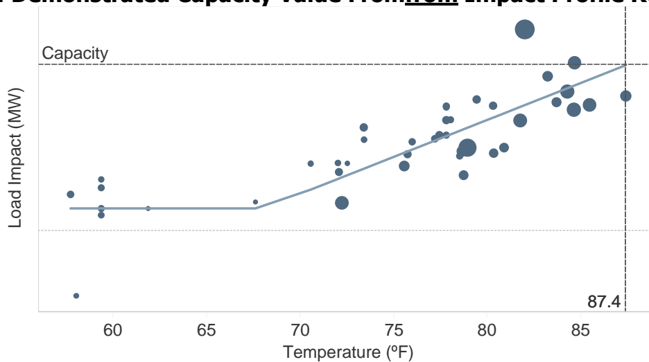
Figure 3: Demonstrated Capacity Value From from Impact-Profile Regression
