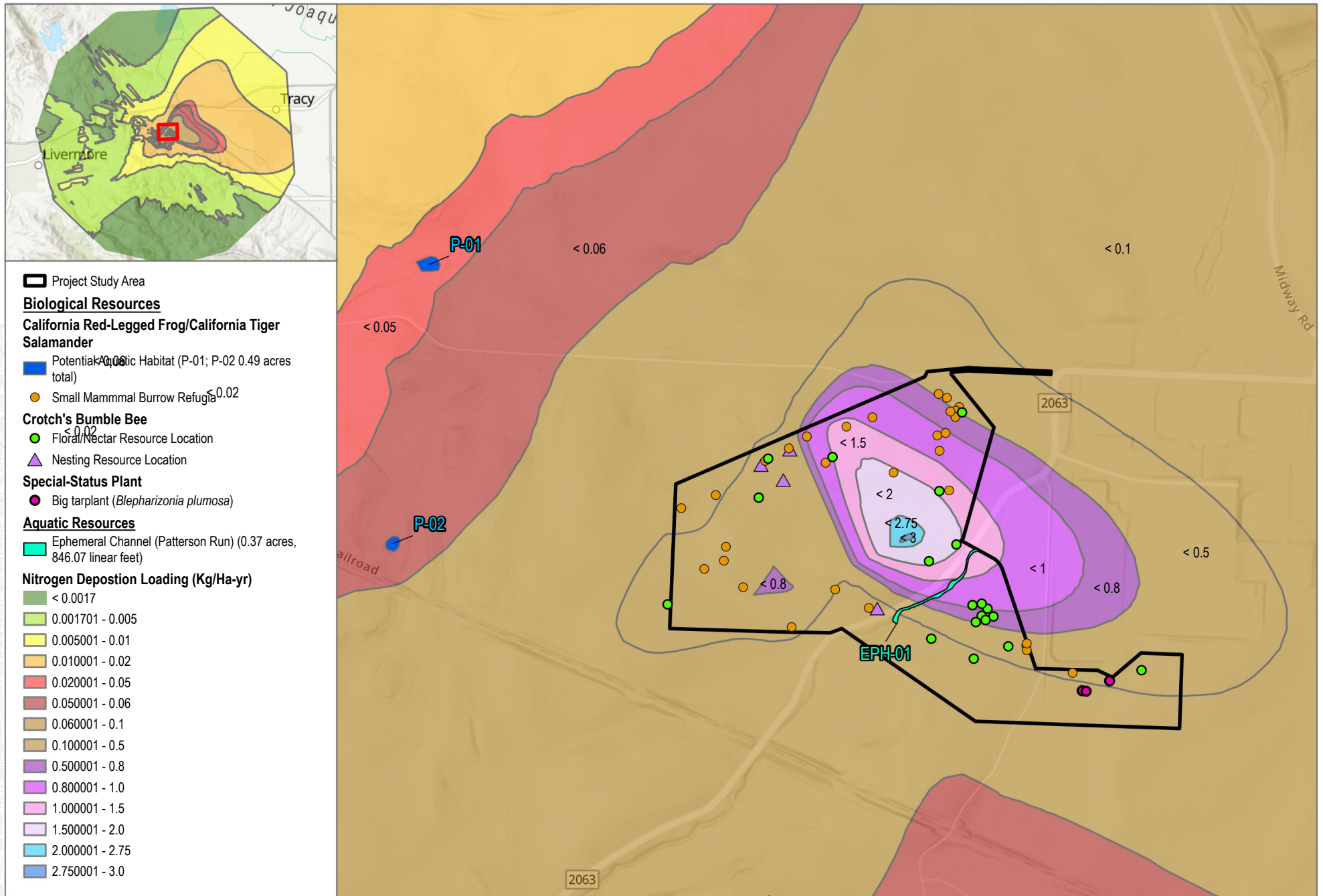
FIGURE 5-3 Biological Resource Nitrogen Deposition Loading Potencia Viridi BESS Project
