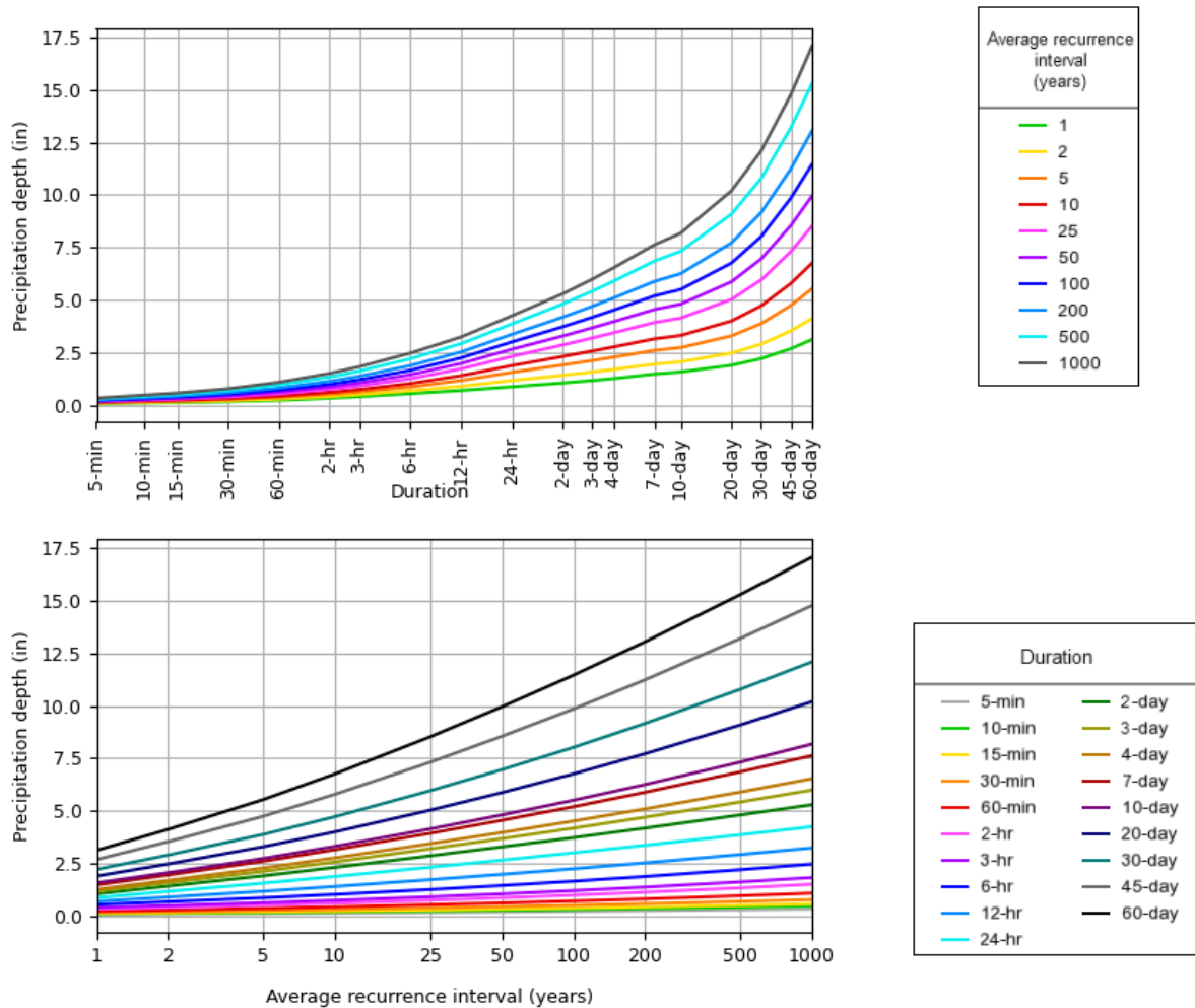
Figure 5.13-13 Depth-Duration-Frequency Curves for Precipitation at the Project Site
