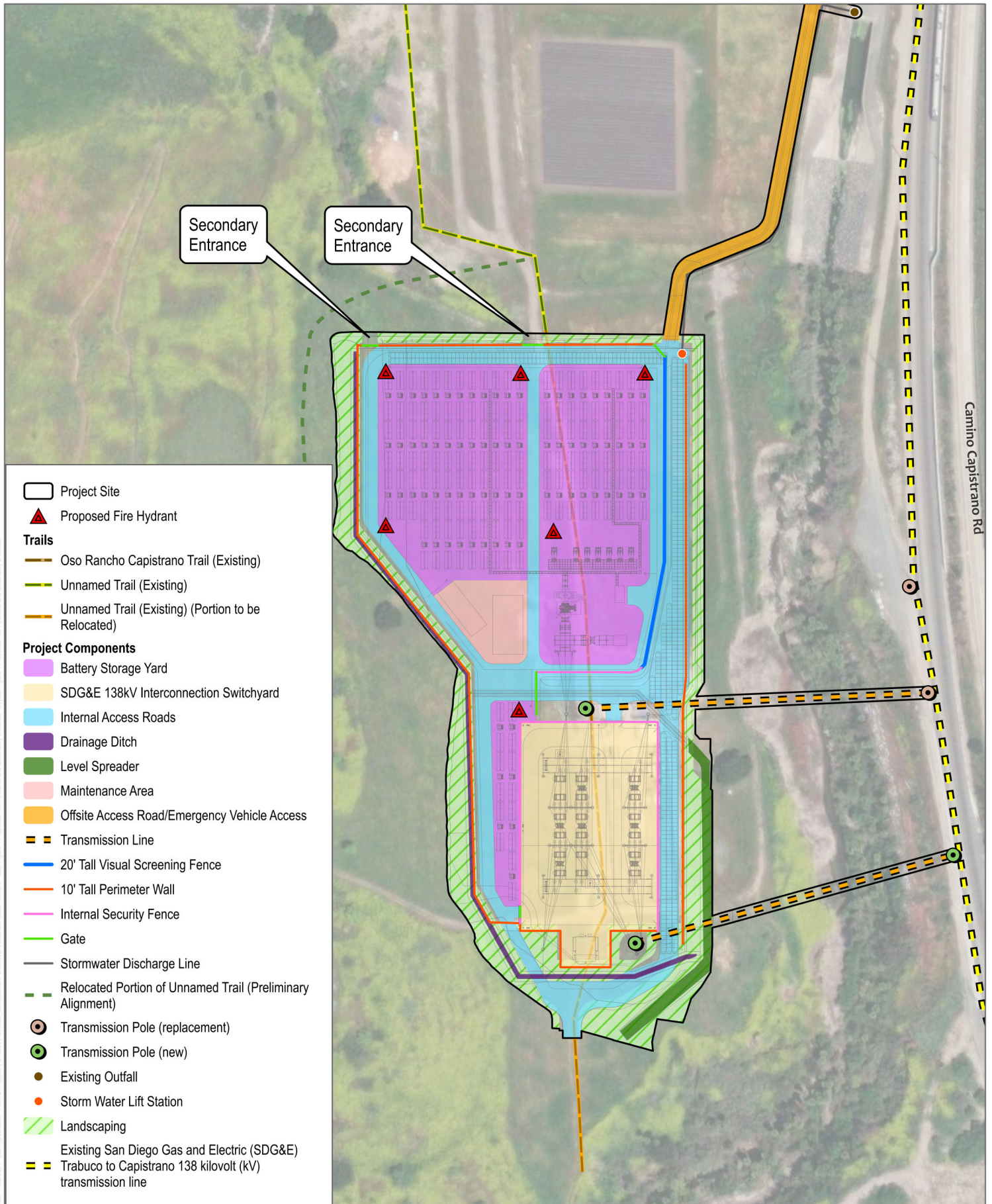
FIGURE 1 Proposed Fire Hydrants and Secondary Entrance
