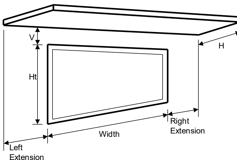
Figure 151514 151514: Overhang Dimensions
