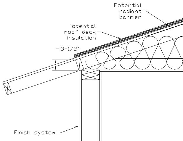
Figure 18 17 : Section at Attic Edge with Standard Truss
