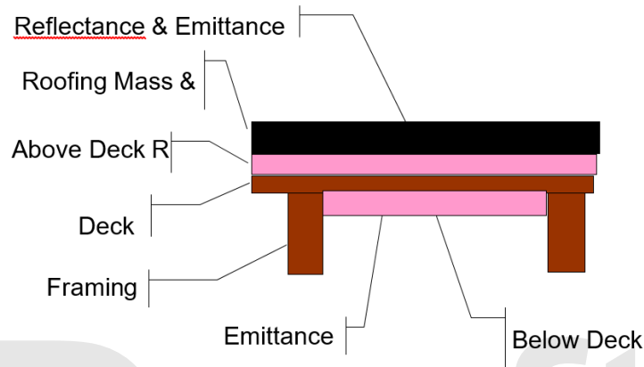
Figure 20202019 2019: Components of the Attic Through Roof Deck
