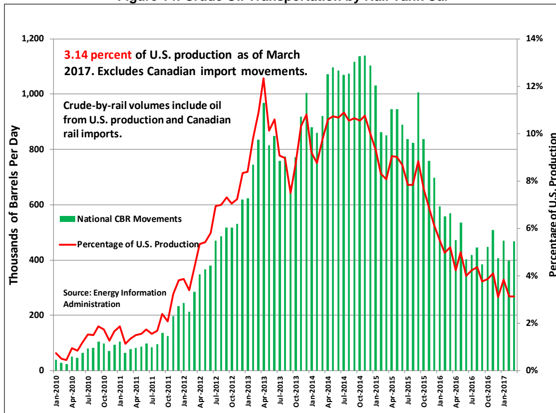
Figure 14: Crude Oil Transportation by Rail Tank Car
