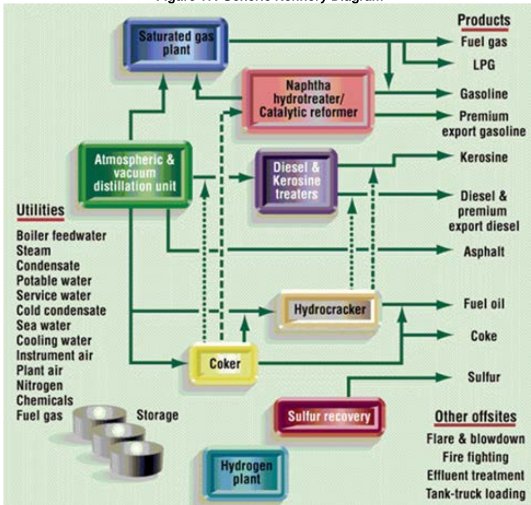
Figure 17: Generic Refinery Diagram
