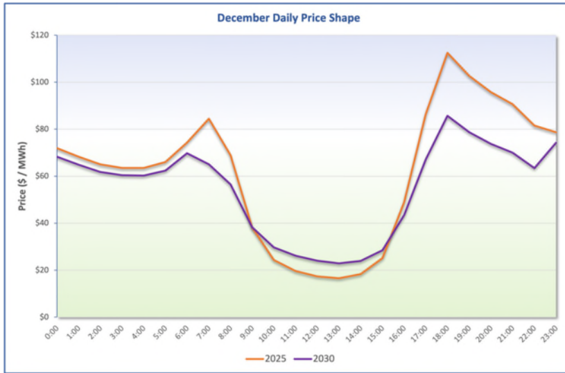
Figure 27. Projected December Daily Price Shapes
