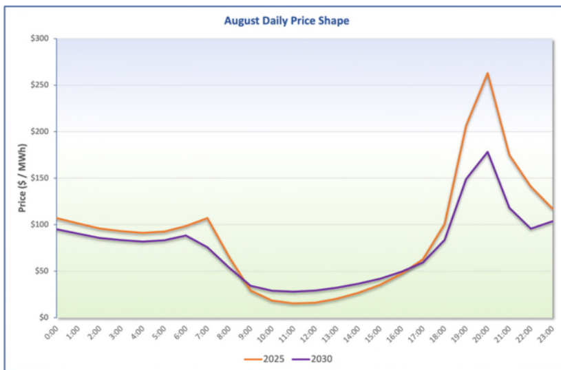
Figure 26. Projected August Daily Price Shapes
