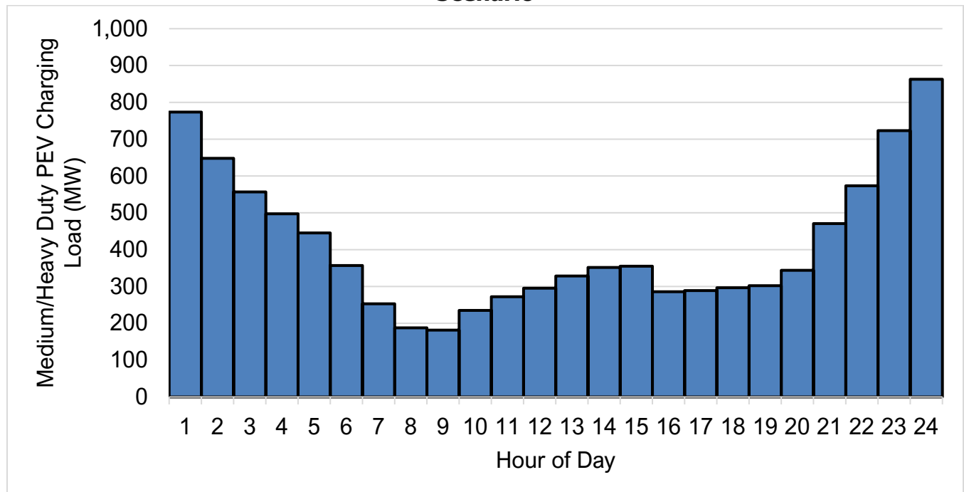
Figure H-1: EAD Load Curve from MDHD BEV Charging in 2030 under AATE3 Scenario
