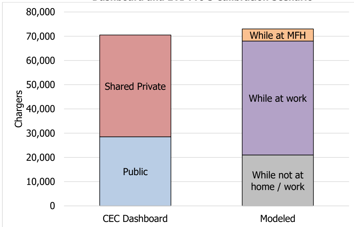
Figure 18: Shared Charging Comparison Between CEC Counting Chargers Dashboard and EVI-Pro 3 Calibration Scenario
