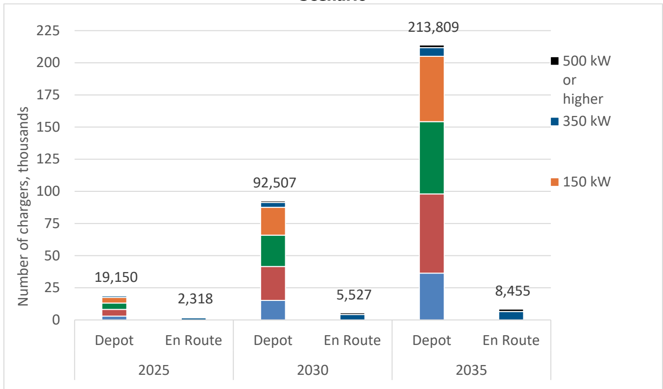
Figure 28: Projected Charging Infrastructure Needs for On-Road Medium- and Heavy-Duty Electric Vehicles Under the High-Speed Depot Alternative Future Scenario
