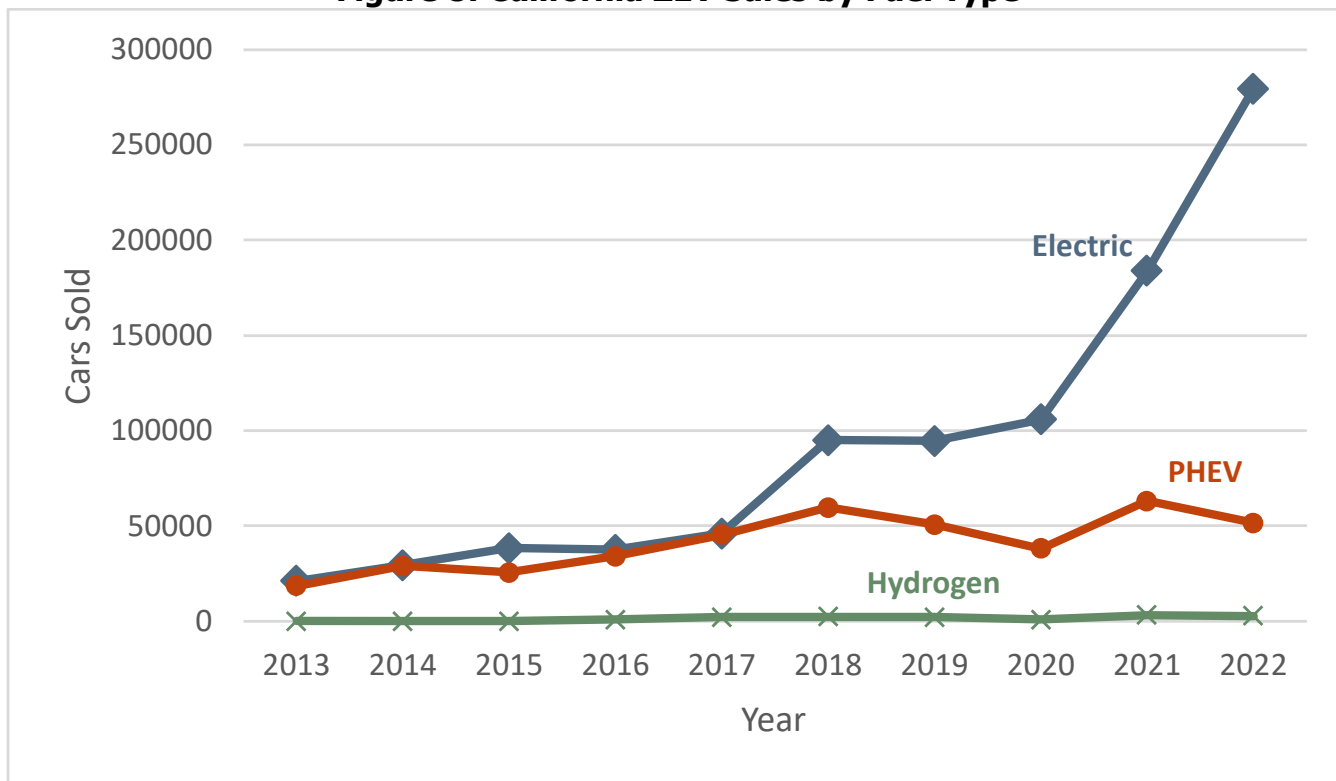
Figure 8: California ZEV Sales by Fuel Type
