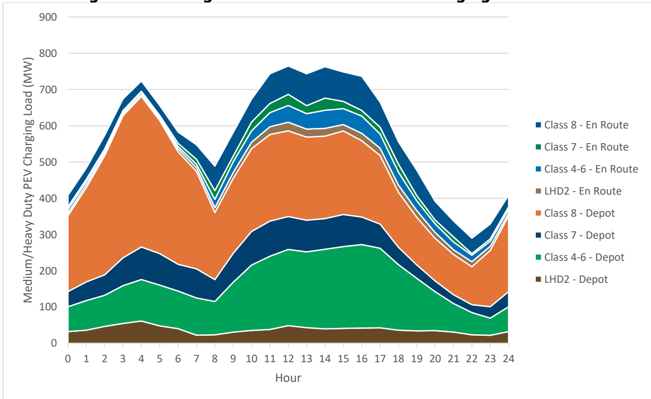
Figure 30: Managed 2030 Statewide MDHD Charging Load Profile
