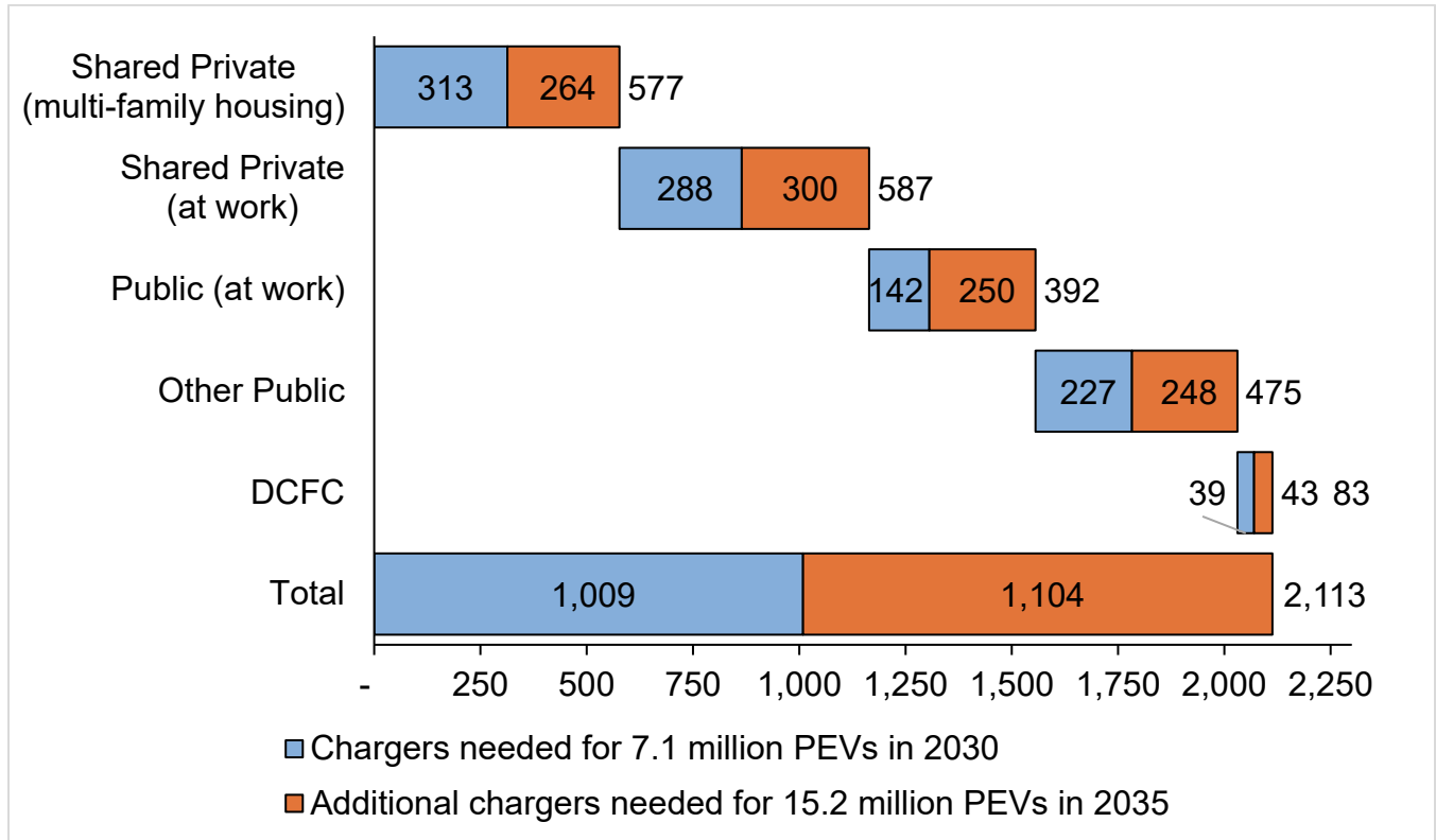
Figure 1: Chargers Needed for Light-Duty Plug-In Electric Vehicles in 2030 and 2035
