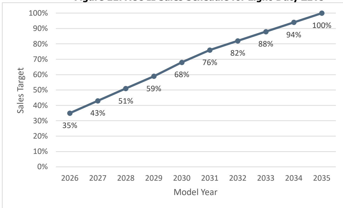
Figure 11: ACC II Sales Schedule for Light-Duty ZEVs
