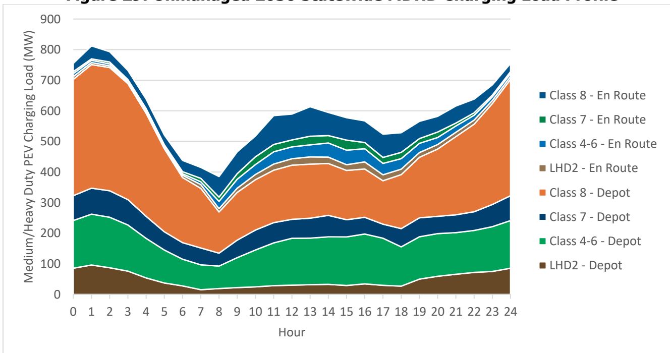
Figure 29: Unmanaged 2030 Statewide MDHD Charging Load Profile
