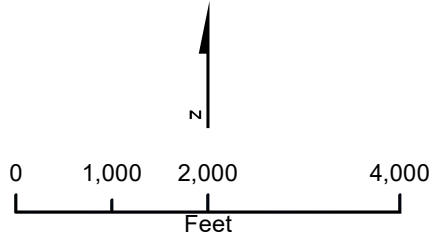
Figure 6b Black Rock Geothermal Project Burrowing Owl Survey Results Imperial County, California
