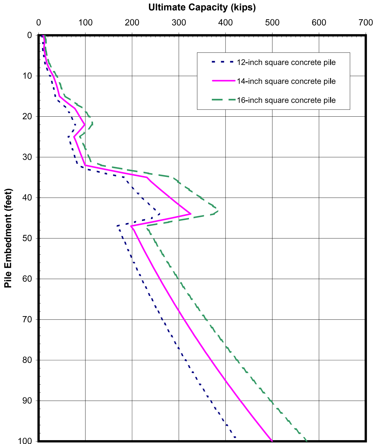
ULTIMATE AXIAL PILE CAPACITY Black Rock Units 1, 2 & 3 Calipatria, California
