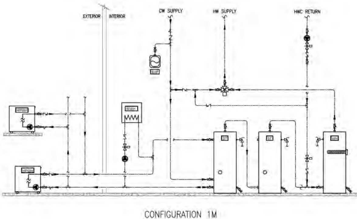
Figure 35: Single-pass primary with electric resistance water heater for temperature maintenance system.
