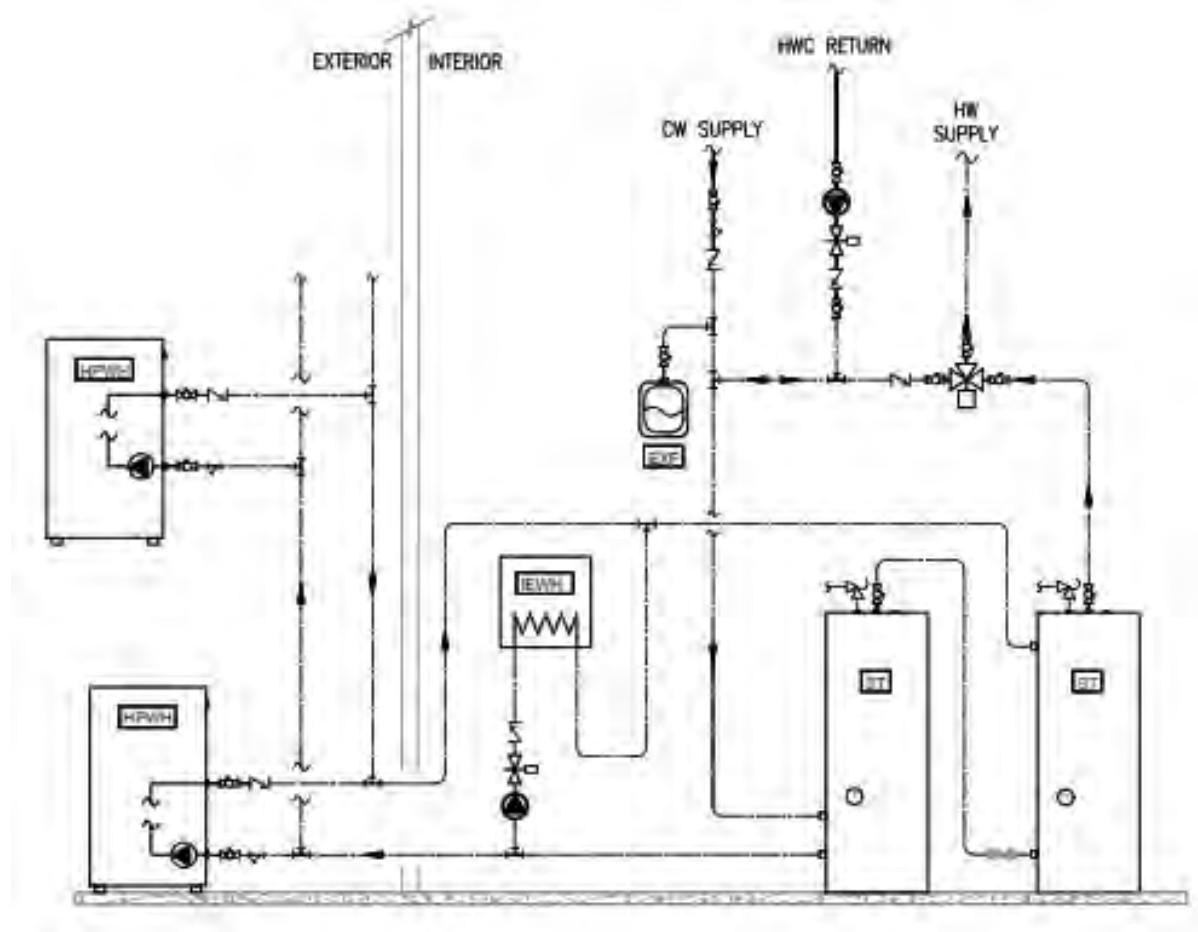
Figure 38: Single-pass return to primary.
