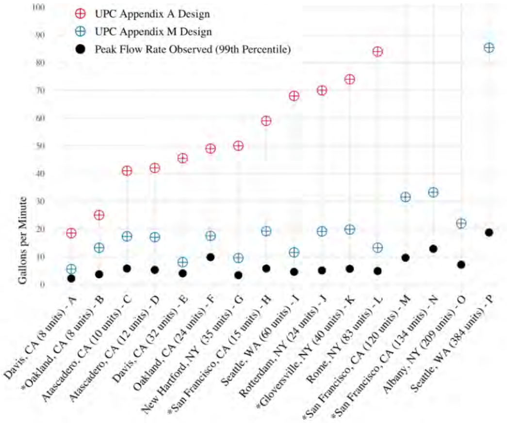
Figure 1: Comparing UPC Appendix A and M design predictions to actual multifamily building peak flow rates.
