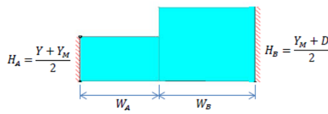
Figure 29: Standard-Heel 1-D Geometry for Insulation Path
