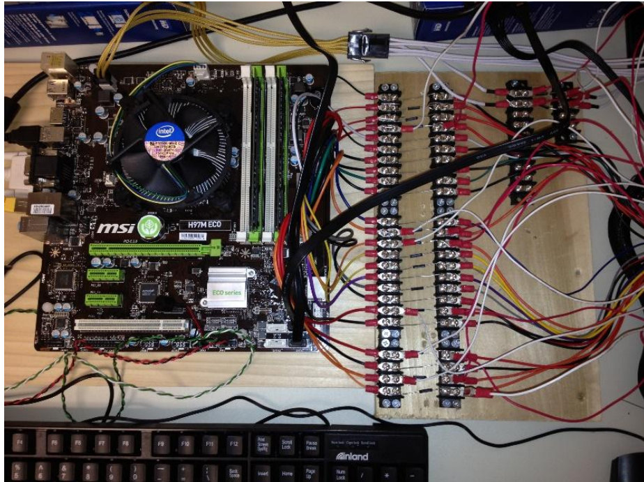
Figure 1. Voltage rails with inserted shunt resistors and measurement wires attached
