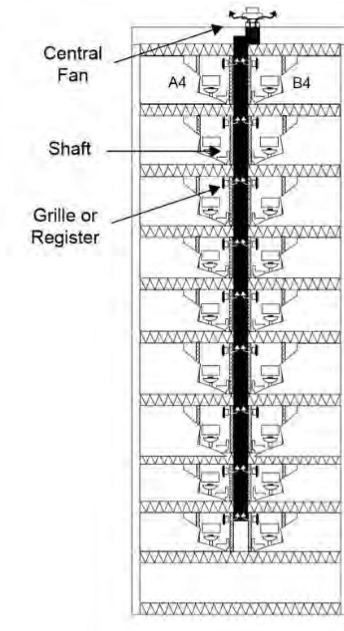
Figure 11-33: Diagram of Central Exhaust Ventilation Duct System Components
