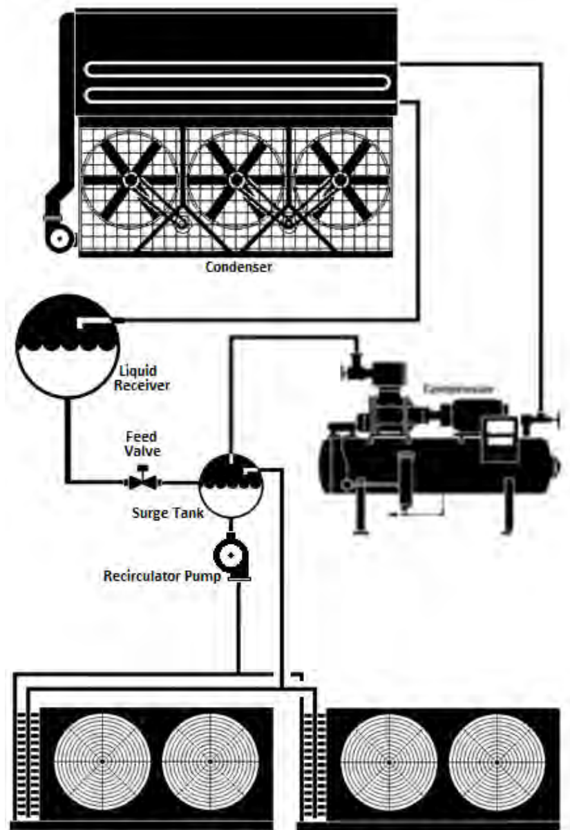
Figure 10-34: Single-Stage System with Pump Recirculated Evaporator Coils
