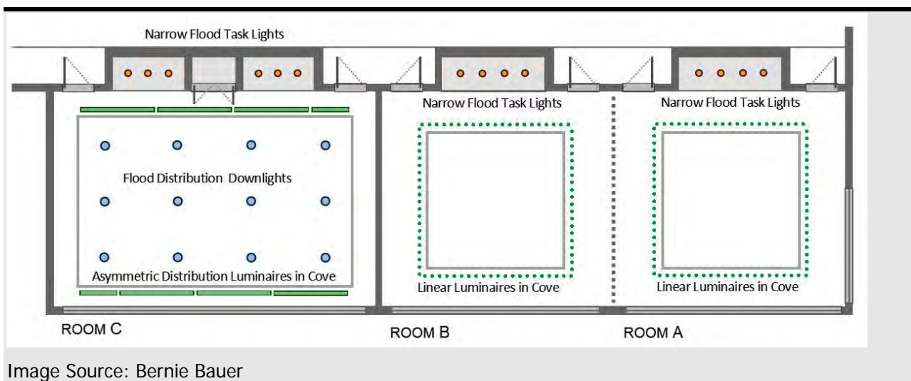
Figure 5-6 Examples of Cove Lighting: Asymmetric Distribution Luminaires in Cove (Room C); Linear Luminaires in Cove (Rooms A and B)
