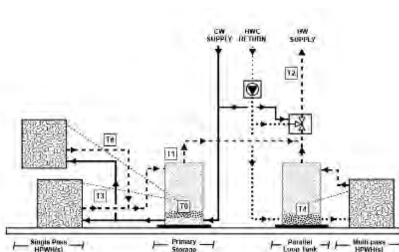
Figure 11-63: Single-Pass HPWH (s) with Parallel Loop Tank
