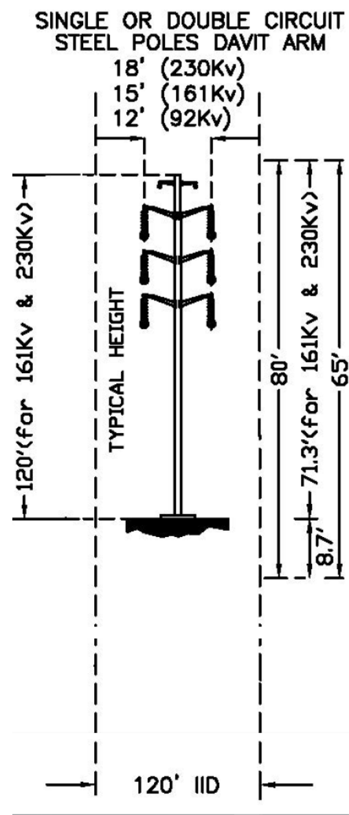
230kv Steel Pole Typical Right of Way
