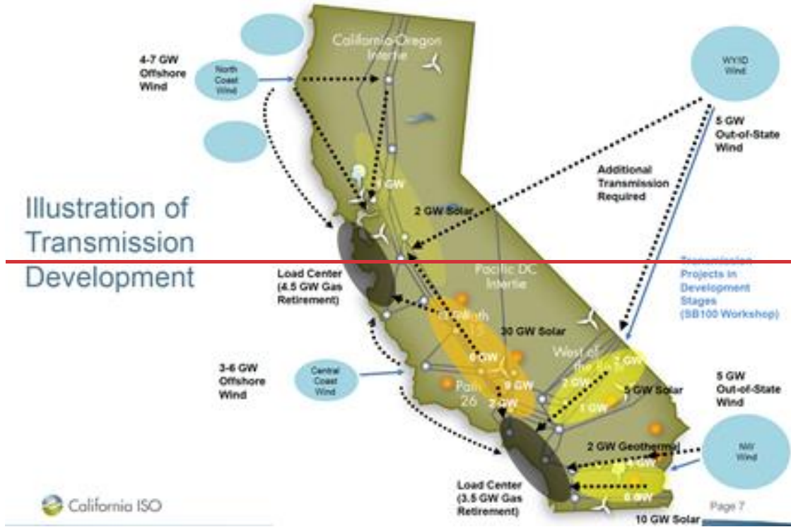
Figure 29291829 1930 : California ISO's Illustrative Transmission Needs From California ISO 20-Year Outlook
