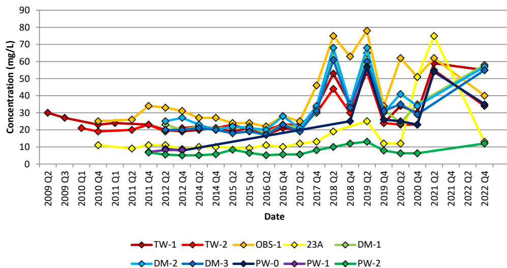
Chart 7: Potassium
