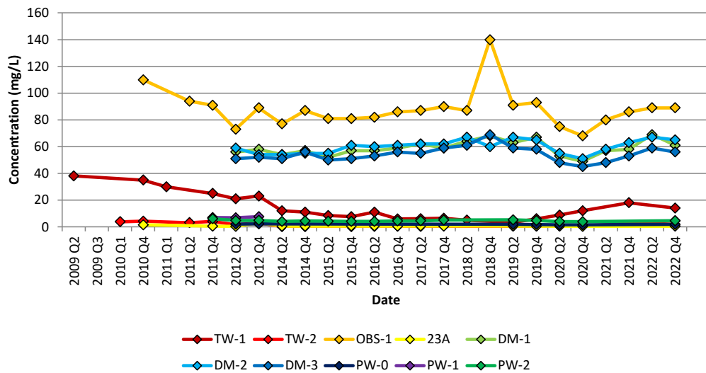
Chart 9: Magnesium
