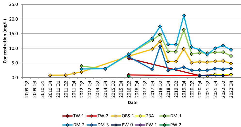
Chart 3: Nitrate (NO 3 )
