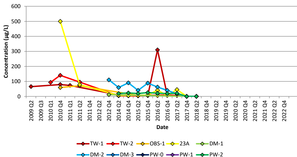
Chart 17: Manganese
