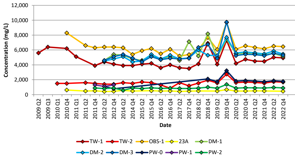
Chart 1: Chloride
