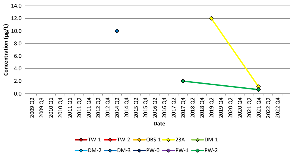
Chart 18: Nickel
