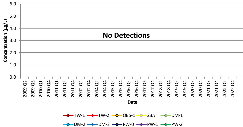
Chart 15: Cobalt
