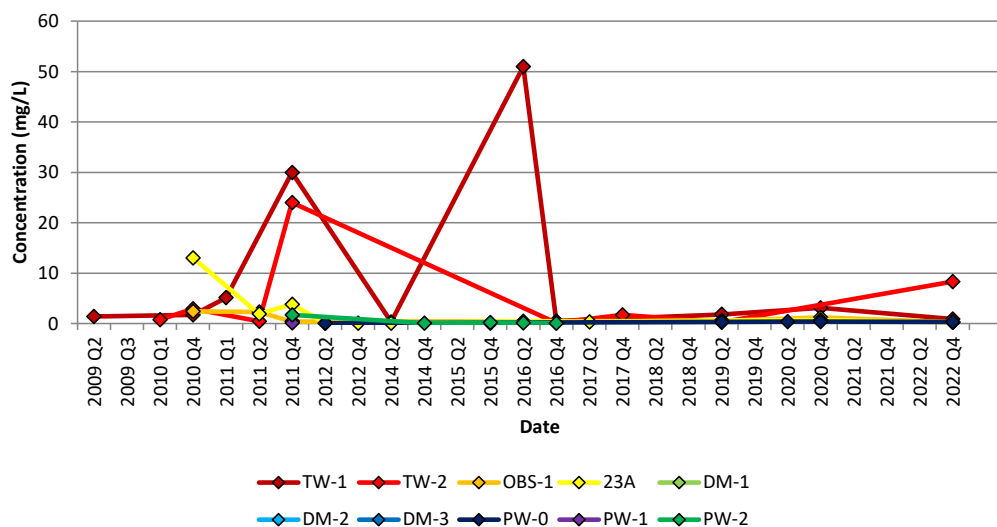
Chart 8: Iron
