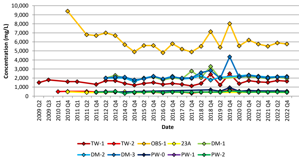
Chart 2: Sulfate (SO 4 )
