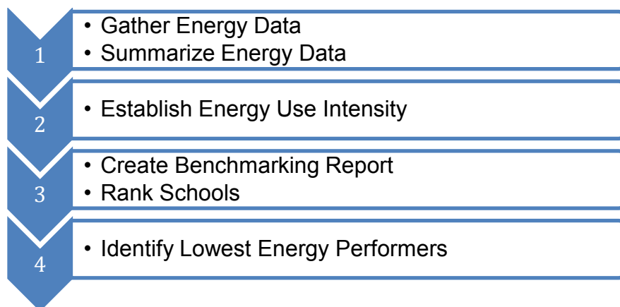
Figure 1: Benchmarking Process
