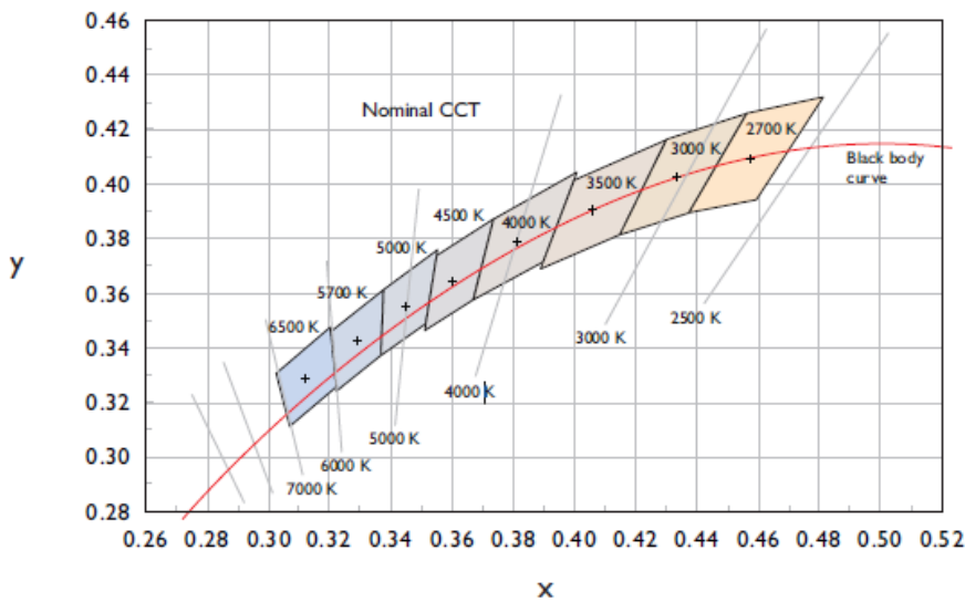
Figure 7 7-step MacAdam Quadrangles on the CIE 1931 Color Space
