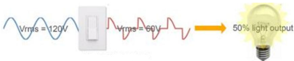
Figure 27 Phase-Cut Dimmer control of incandescent lamp
