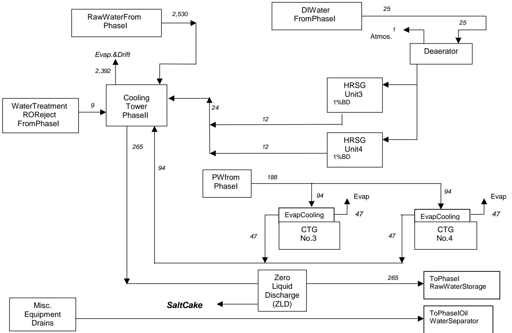
Figure 8.14.3dR Cosumnes Power Project Phasel I – 104F Peak WATER BALANCE DIAGRAM PBPOWER, INC.
