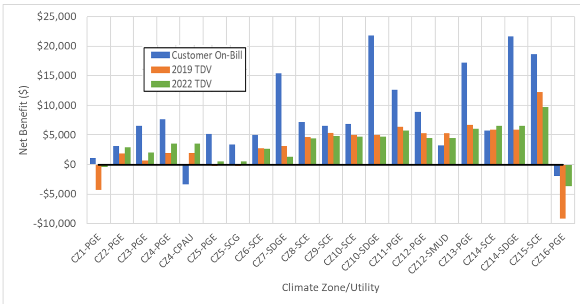
Figure 7: Net benefit – min efficiency heat pump at HVAC replacement + PV + panel upgrade: 1992-2010.
