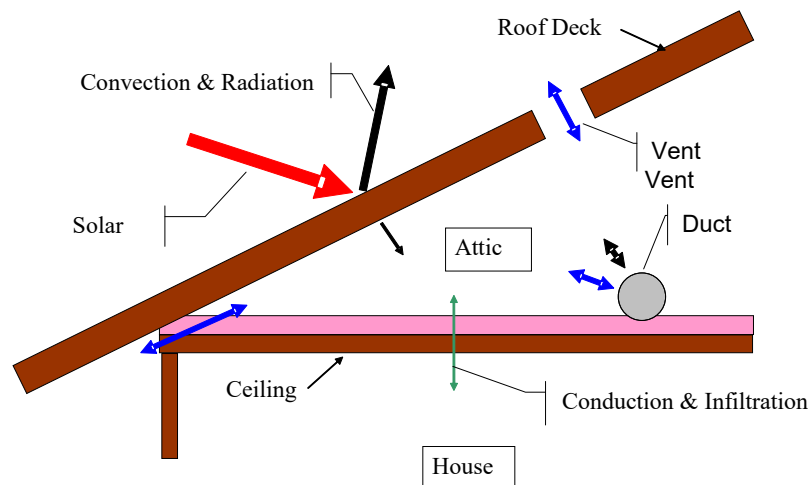
Figure 17: Attic Model Components
