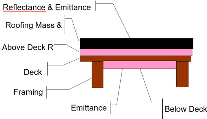
Figure 20: Components of the Attic Through Roof Deck
