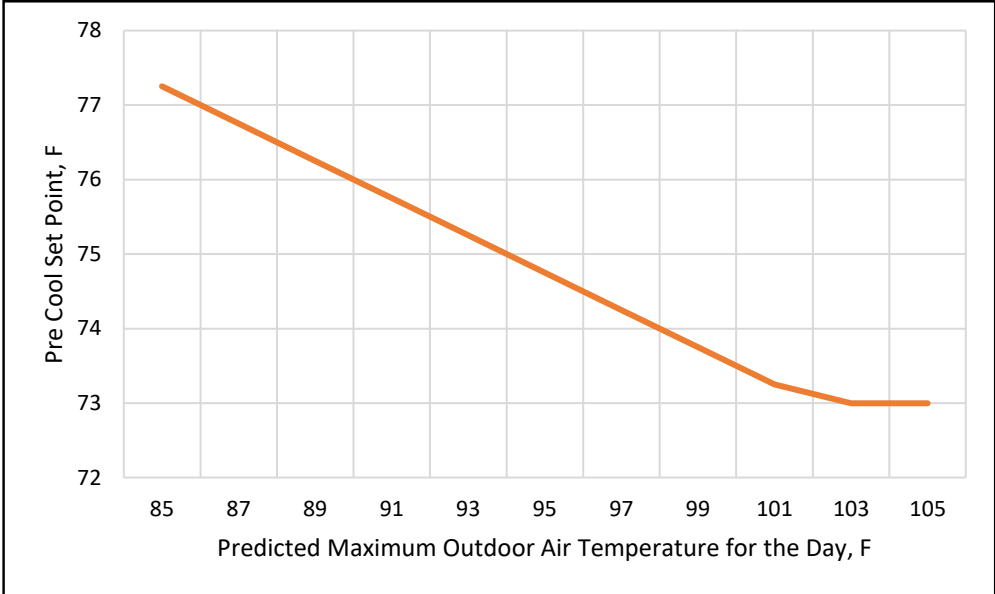
Figure 9: Precooling Thermostat Setpoint
