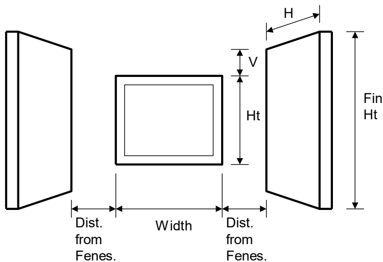
Figure 16: Sidefin Dimensions
