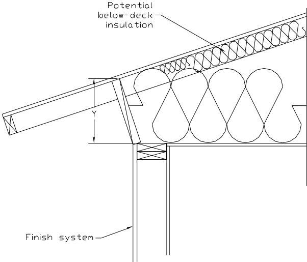
Figure 19: Section at Attic Edge with a Raised Heel Truss
