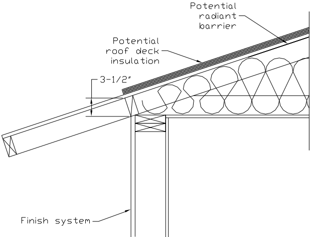
Figure 18: Section at Attic Edge with Standard Truss
