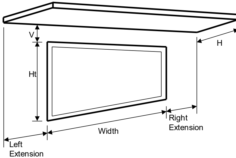
Figure 15: Overhang Dimensions
