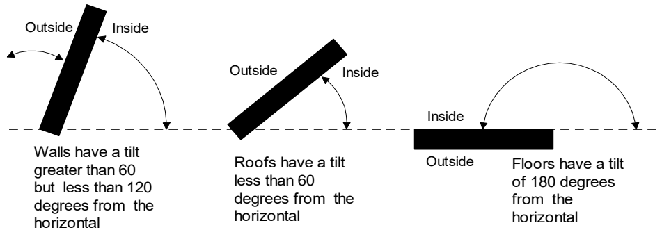
Figure 13: Surface Definitions
