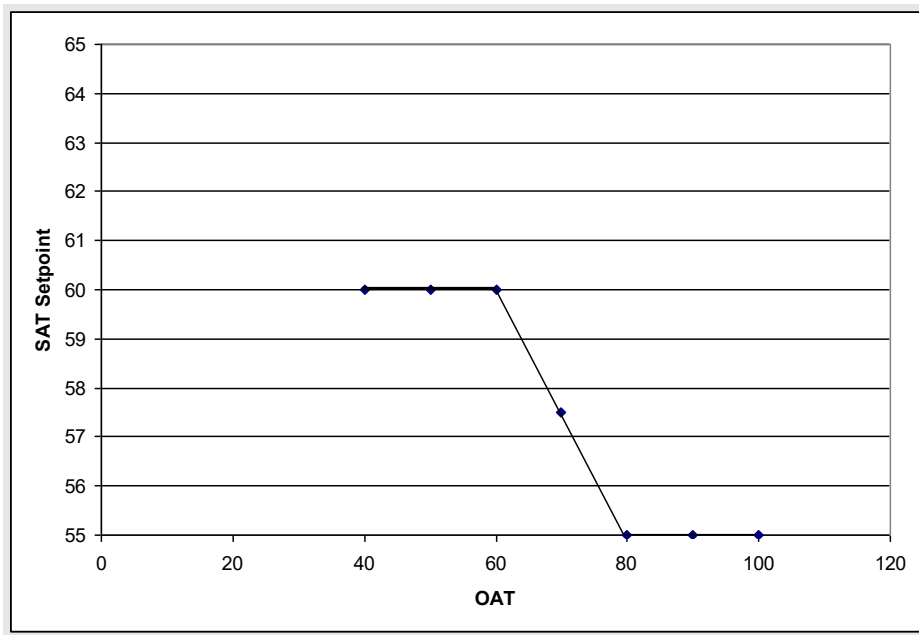
Figure 8: SAT Cooling Setpoint Reset Based on Outdoor Air Temperature (OAT)
