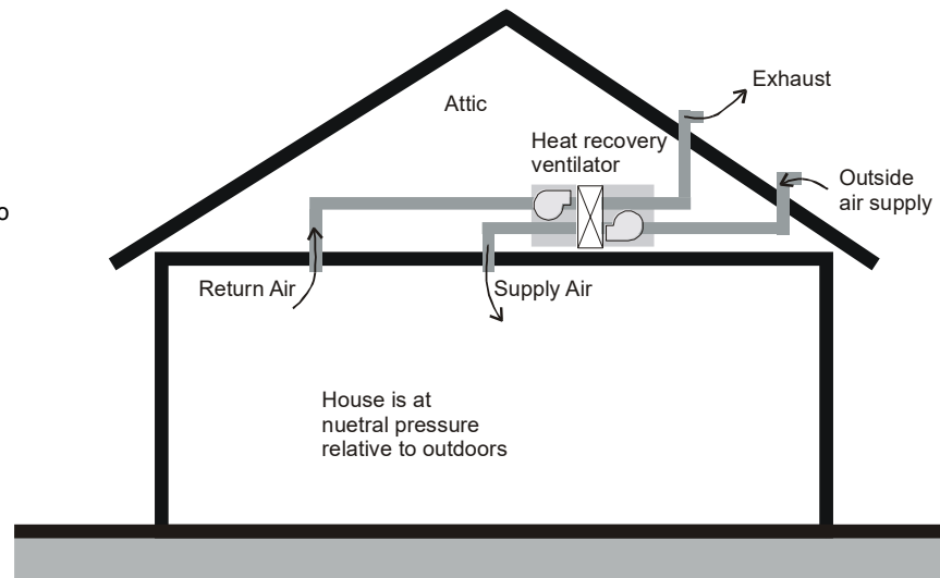
Figure 4-31: Balanced Ventilation Example 1 – HRV or ERV
