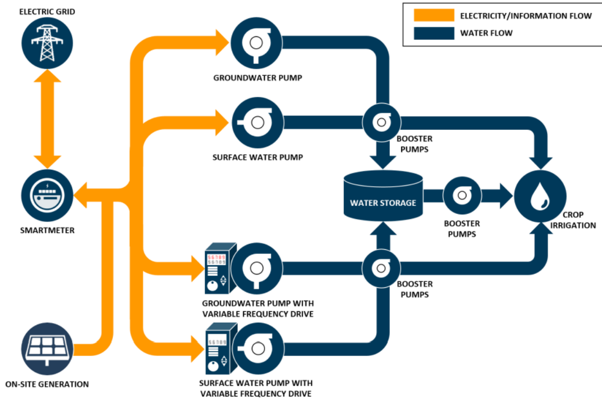
Figure 41: Water Energy Flows in a Typical California Farm
