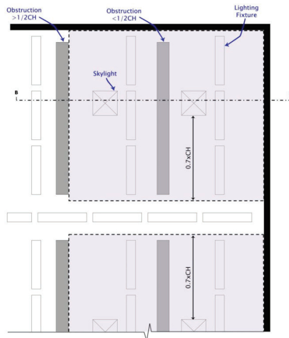
Figure 5-14 An Example of Skylit Daylit Zone Layout – in an Overhead View
