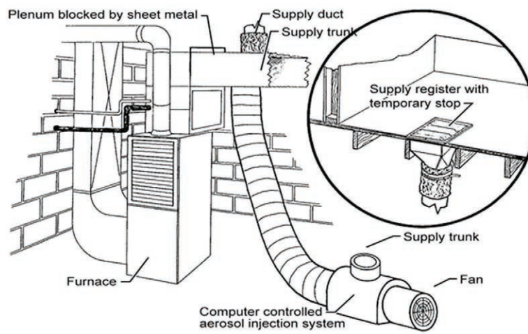
Figure 11-45: Computer-Controlled Aerosol Injection System
