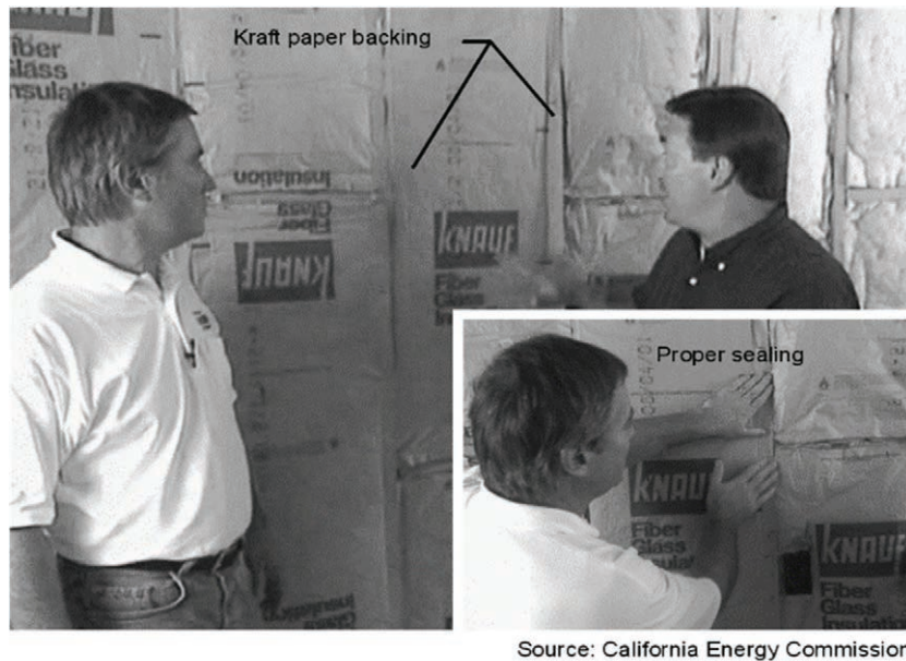
Figure 11-7: Typical Kraft-faced Vapor Retarder Facing
