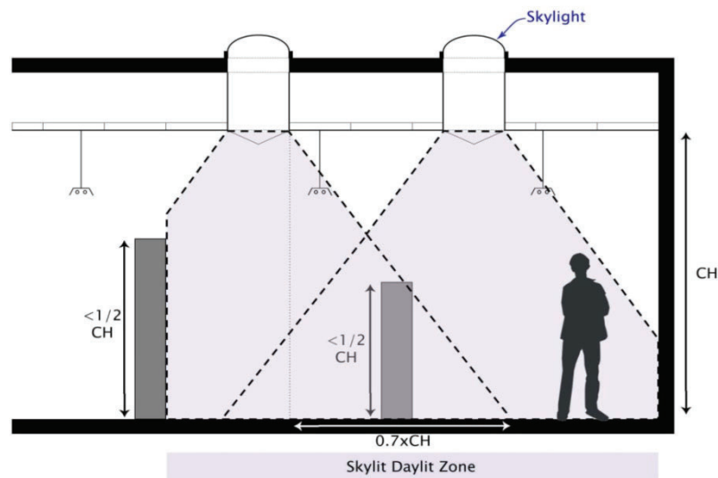
Figure 5-15 An Example of Skylit Daylit Zone Layout - in a Sideview Perspective
