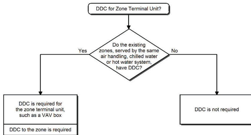
Figure 4-2223: Zone Terminal Unit Flowchart
