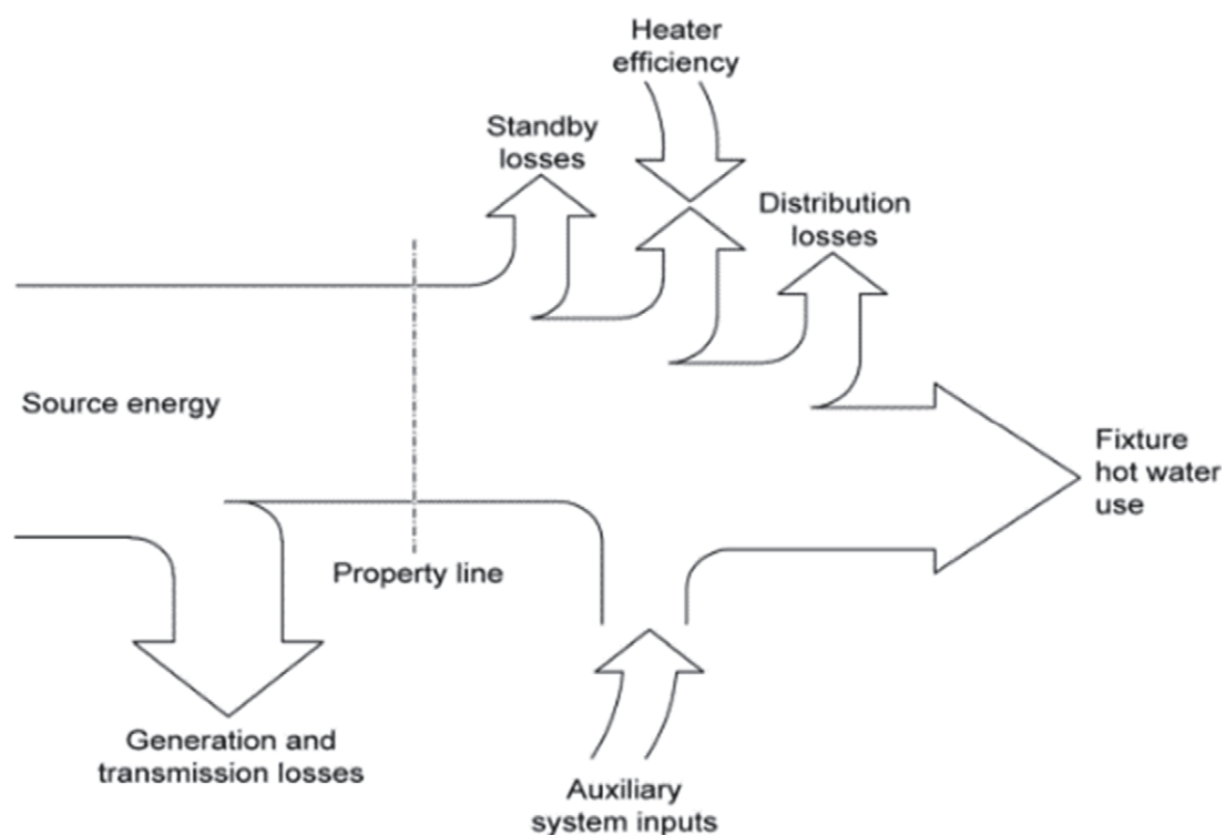
Figure 11-64: Water Heating Energy Flow Representation
