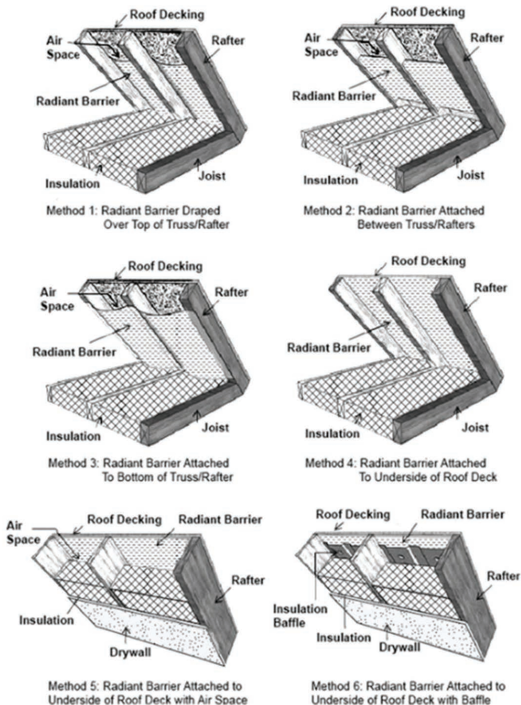
Figure 11-5: Methods of Installation for Radiant Barriers
