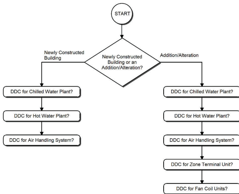
Figure 4-1849: Building Status Flowchart
