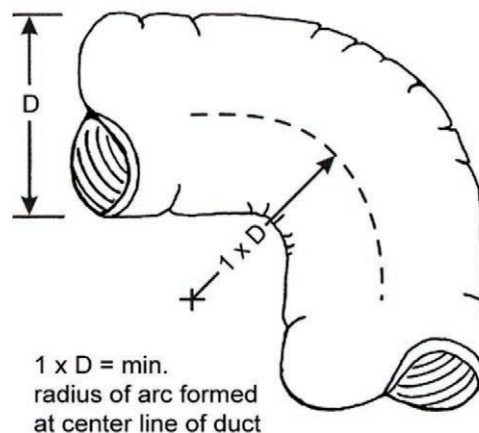
Figure 11-44: Minimizing Radius for Flex Duct Bends
