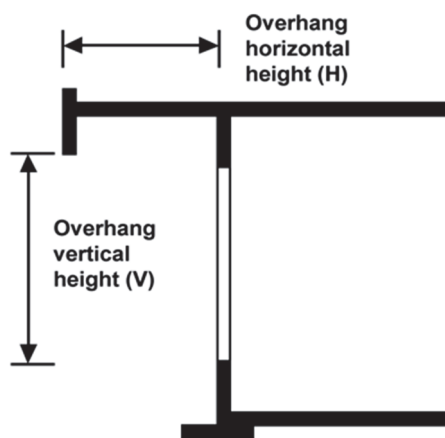
Figure 3-14: Overhang Dimensions
