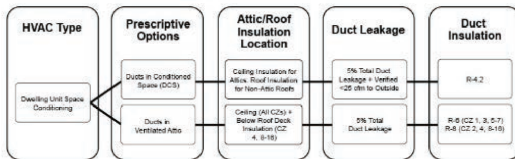
Figure 11-52: Duct Prescriptive Compliance Choices
