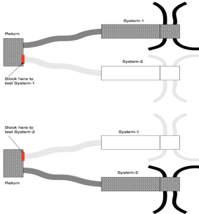
Figure 4-1342: Example of Two Duct Systems with a Common Return
