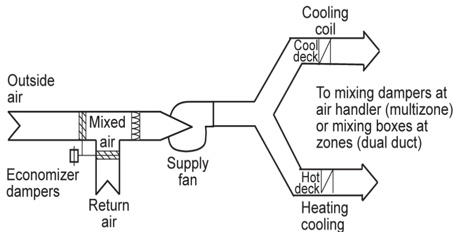
Figure 4-2829: Single-Fan Dual-Duct System
