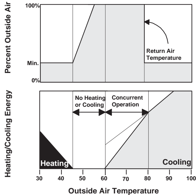
Figure 4-3536: Integrated Air Economizer
