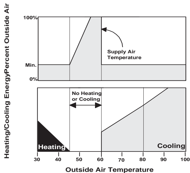
Figure 4-3637: Nonintegrated Air Economizer
