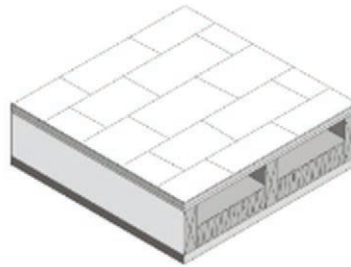
Figure 24: 2nd and 4th: Deck Roofs (2022 Ref. App. Fig. 4.2.2)
