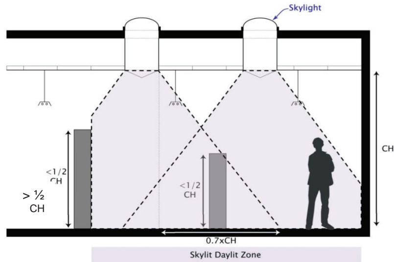
Figure 5-15: Skylit Daylit Zone Diagram 2
