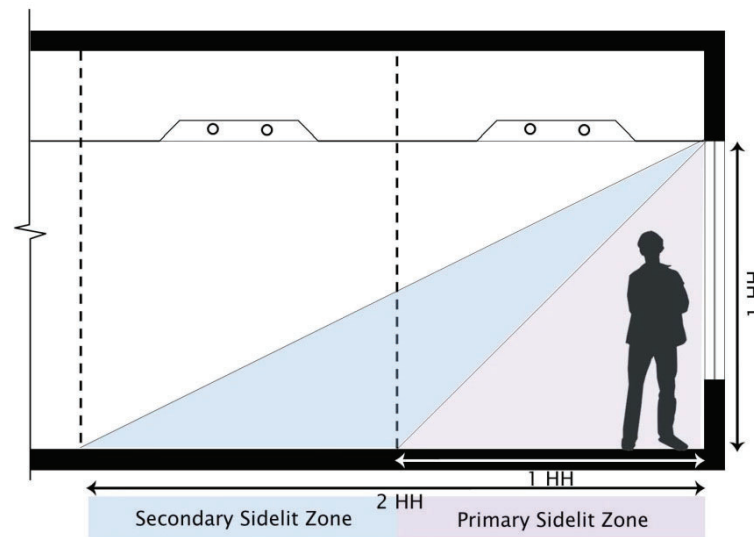
Figure 5-12: Secondary Sidelit Daylit Zone Diagram Figure 5-18 Example of Secondary Sidelit Daylit Zone (in a sideview)
