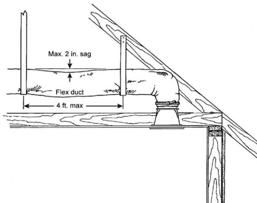
Figure 11-42: Minimum Spacing for Suspended Flex Ducts
