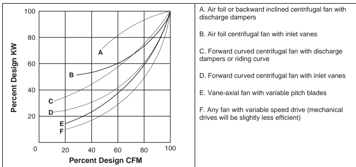
Figure 4-2930: VAV Fan Performance Curve
