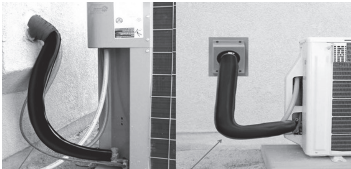
Figure 11-37: Refrigerant Line Insulation
