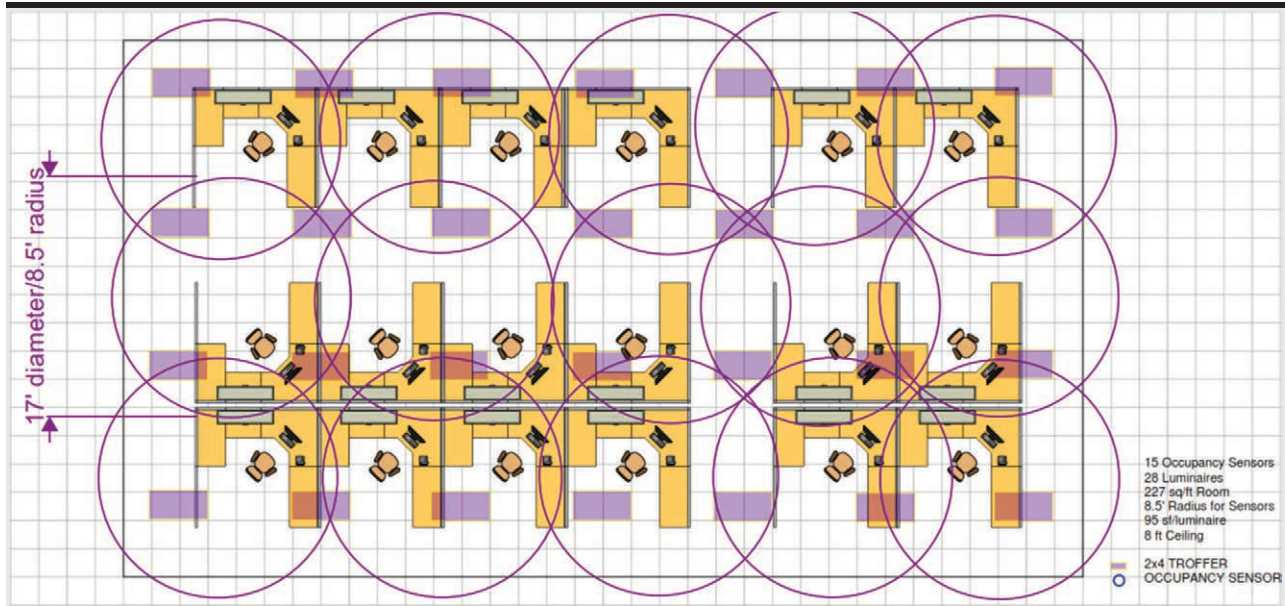
Figure 5-11 (for Example 5-7) An Office Plan with Occupant Sensing Control Zone Layout
