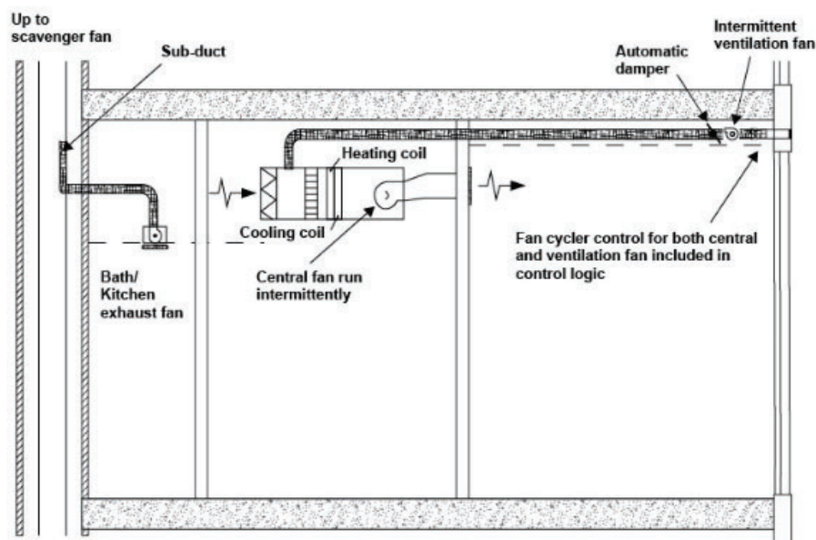
Figure 11-32: Example of Central Fan-Integrated (CFI) Ventilation with MERV 13 Filtration
