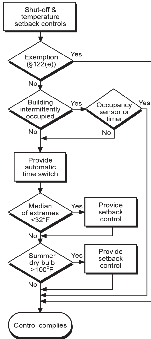
Figure 4-1647: Shut-Off and Setback Controls Flowchart
