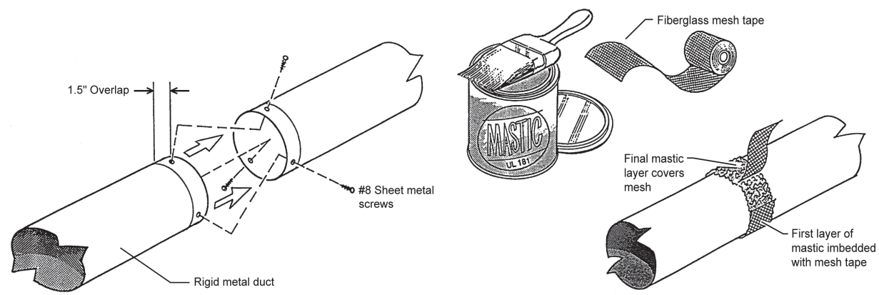
Figure 11-39: Sealing Metallic Ducts with Mastic and Mesh
