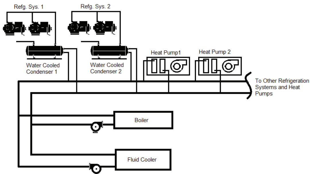
Figure 10-19: Water Loop Heat Pump Example
