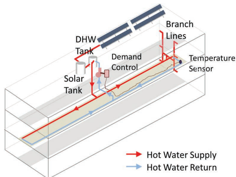
Figure 4-3334: Example of a Dual-Loop Recirculation System
