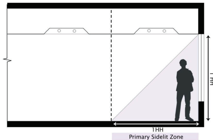
Figure 5-17 Example of Primary Sidelit Daylit Zone Layout (in a sideview)
