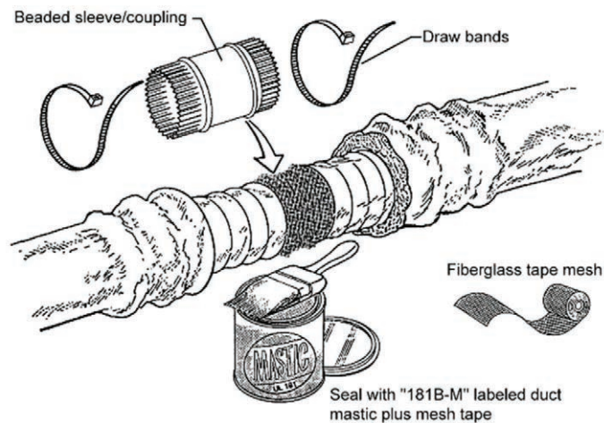
Figure 11-47: Connecting Flex Ducts Using Mastic and Mesh
