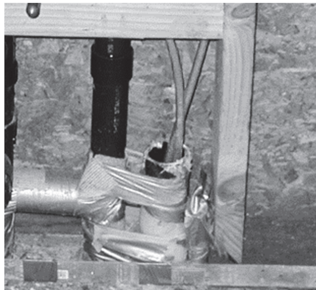
Figure 11-76: Noncompliant Below-Grade Piping and Hot and Cold Water Lines Separation
