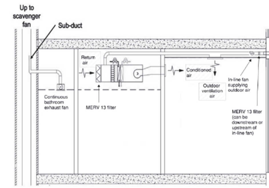
Figure 11-27: MERV 13 Locations for Ventilation and Space Conditioning Air Handler Unit in Example Scenario
