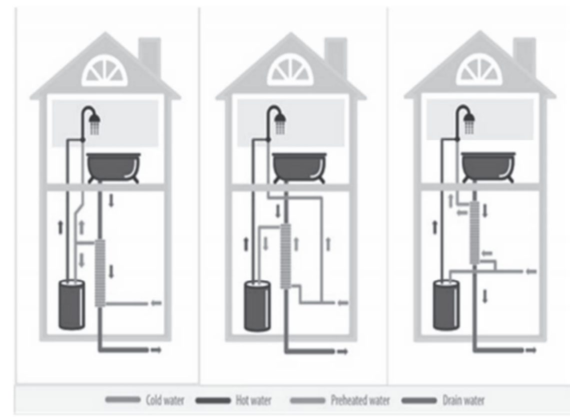
Figure 11-70: The Three Plumbing Configurations of DWHR Installation (From left to right: Equal Flow, Unequal Flow - Water Heater, Unequal Flow - Fixture)
