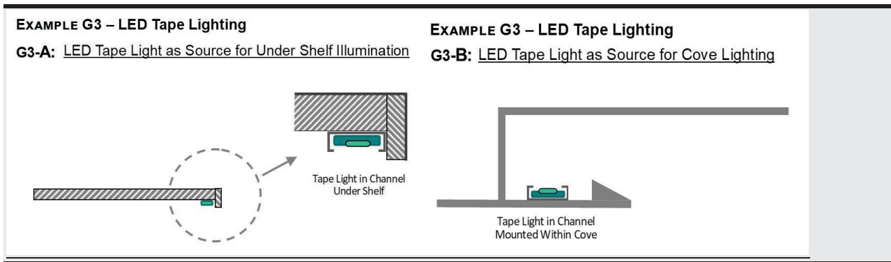
Figure 5-5 Examples of LED Tape Lighting in Applications: In use as under shelf lighting (left image); In use as Cove Lighting (right image)
