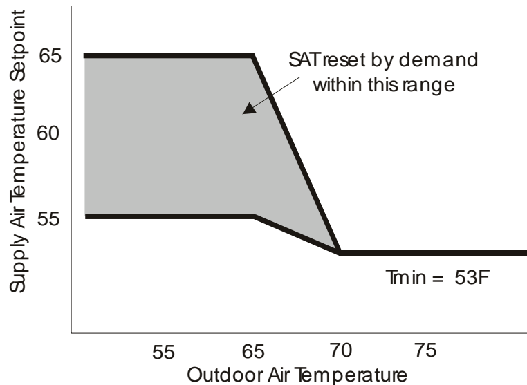
Figure 4-3034: Energy Efficient Supply Air Temperature Reset Control for VAV Systems
