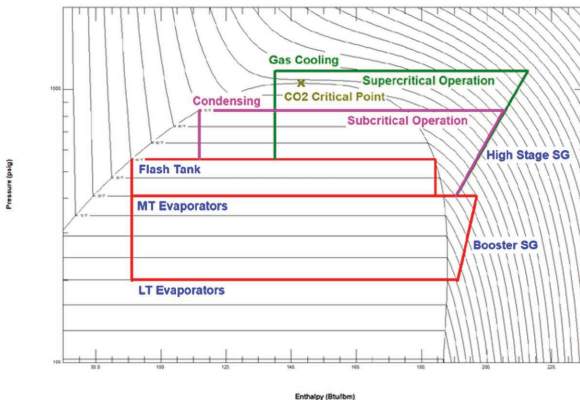
Figure 10-38: Common Transcritical CO 2 System Configuration
