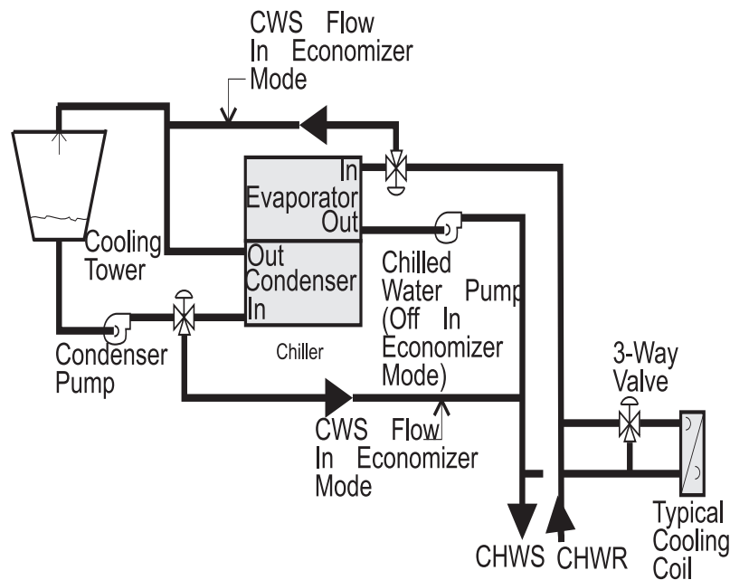
Figure 4-3738: “Strainer-Cycle” Water Economizer
