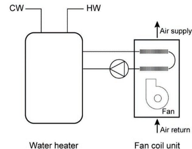
Figure 11-55: Combined Hydronic System with Water Heater as Heat Source
