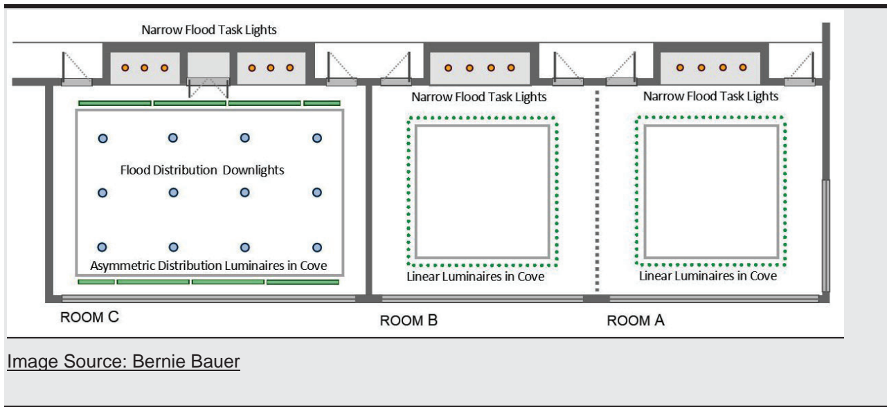
Figure 5-6 Examples of Cove Lighting in Applications: Asymmetric Distribution Luminaires in Cover (left image); Linear Luminaires in Cove (center image & right image)
