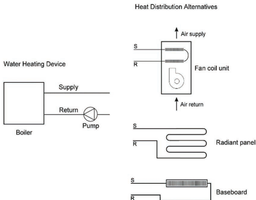
Figure 11-54: Hydronic Heating System Components
