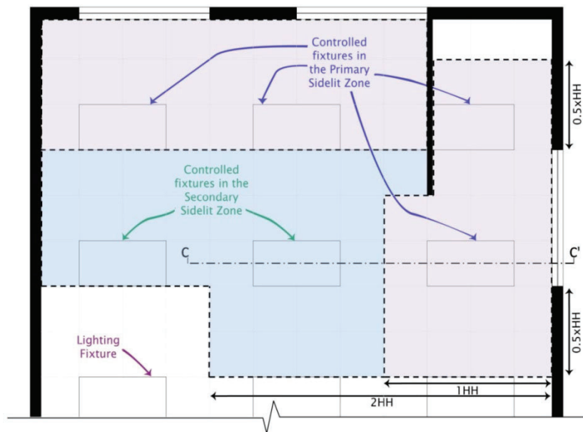
Figure 5-19 Example of Secondary Sidelit Daylit Zone (in an overhead view)
