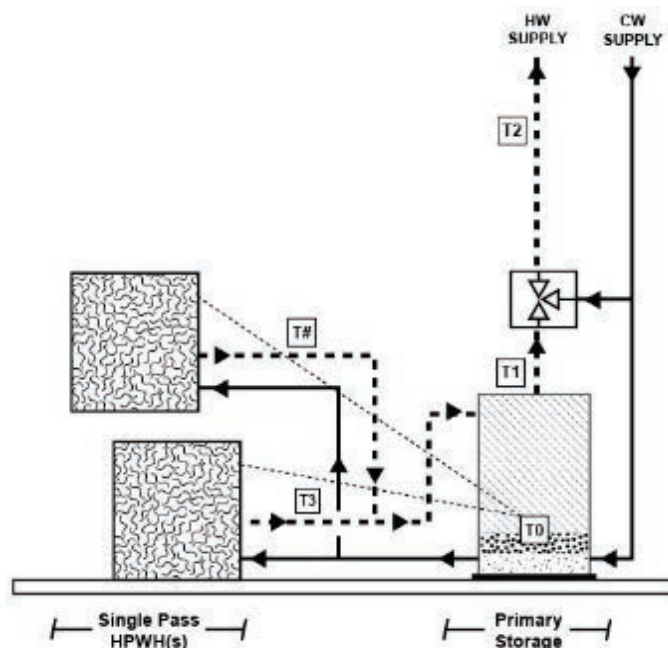
Figure 11-69: Single-Pass HPWH(s) without Hot Water Recirculation (For Clustered Design)
