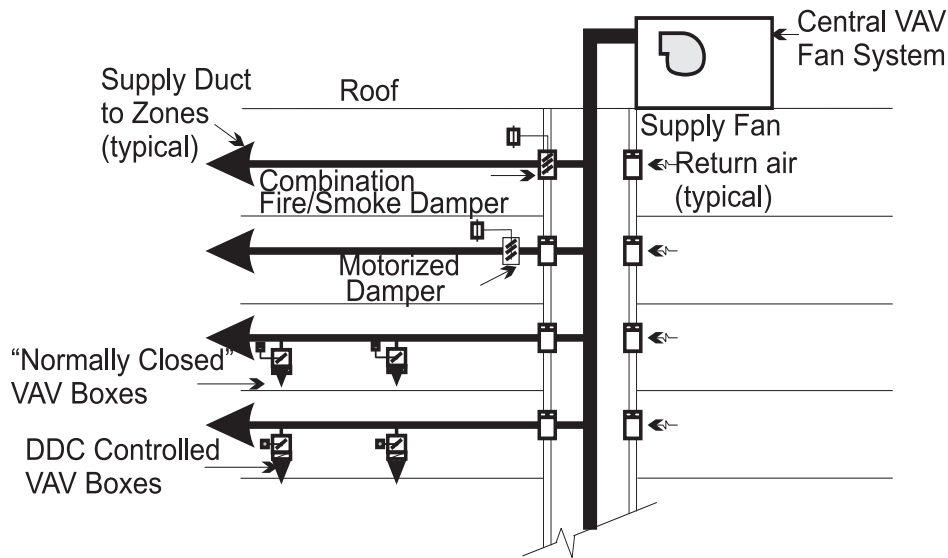
Figure 4-1748: Isolation Methods for a Central VAV System
