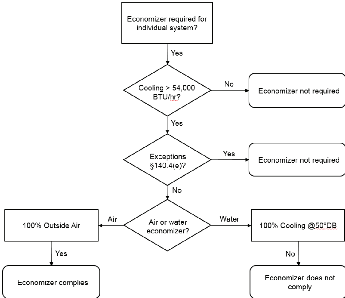
Figure 4-2728: Economizer Flowchart
