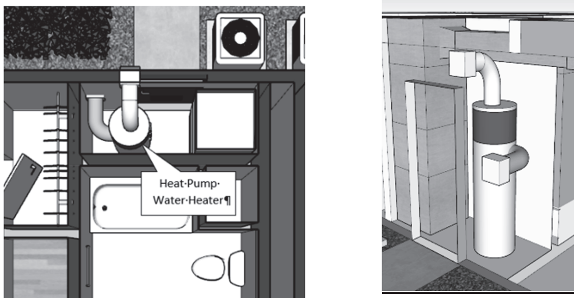
Figure 78: Garden Style Multifamily Case Study: Heat Pump Water Heater in Closet with Ducts to Outside
