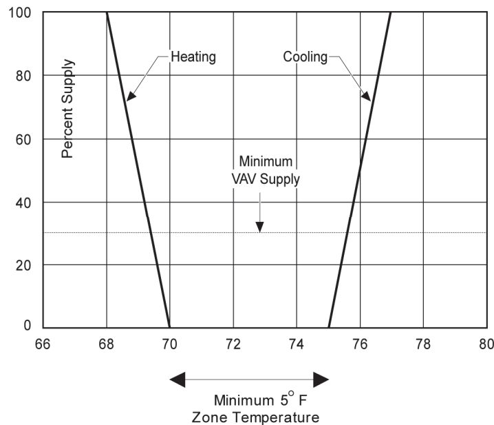
Figure 4-1413: Proportional Control Zone Thermostat
