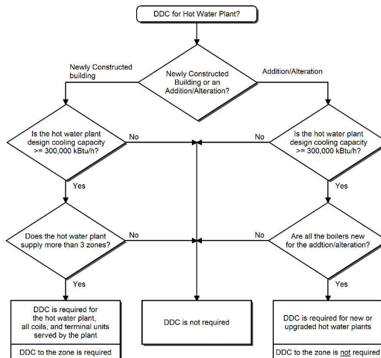
Figure 4-2024: Hot Water Plant Flowchart
