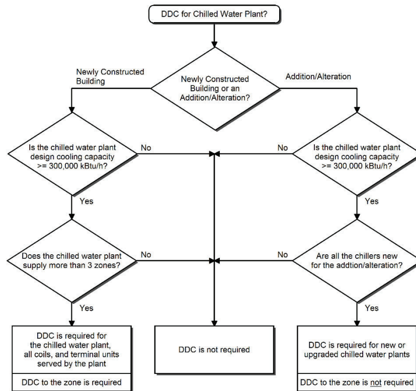
Figure 4-1920: Chilled Water Plant Flowchart
