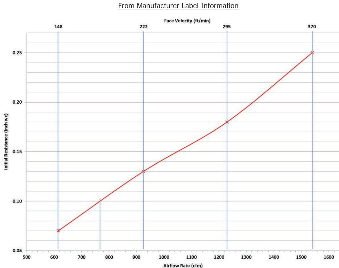
Figure 11-50: Plot of Pressure drop vs. Airflow for a 20" X 30" X 1" Depth Air Filter
