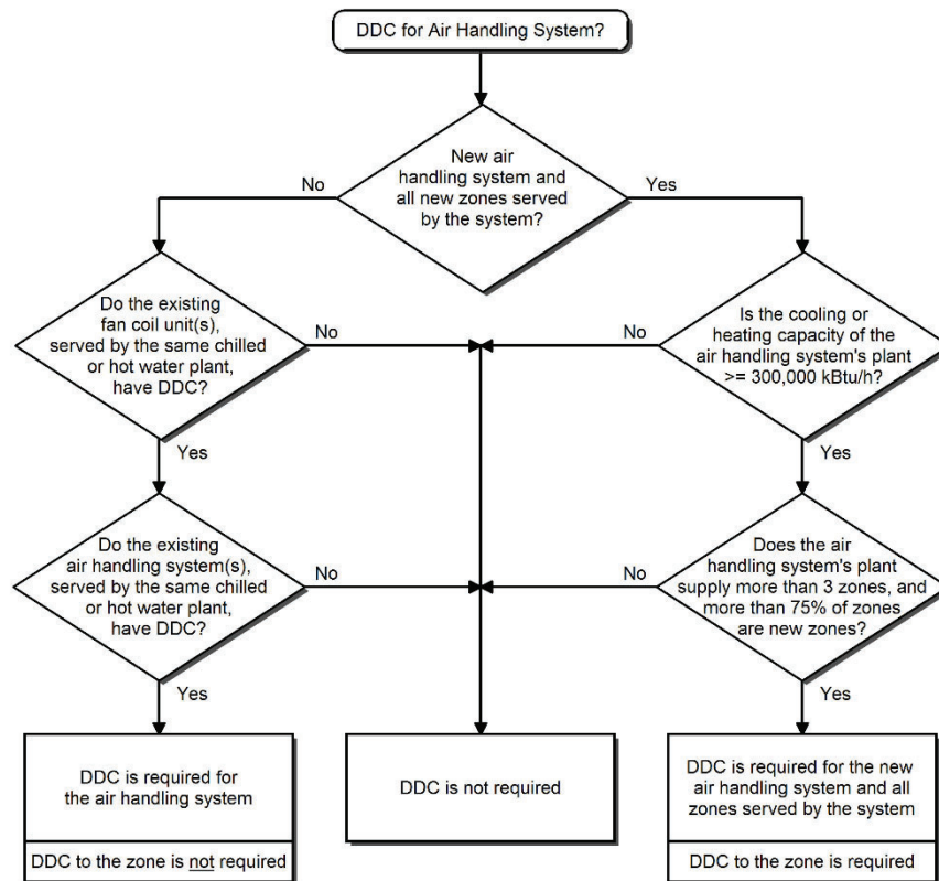
Figure 4-2122: Air Handling System Flowchart
