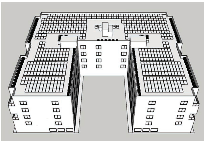
Figure 85: Mid-Rise Multifamily Case Study: Photovoltaics (PV) on Flat Roof (viewed from South)
