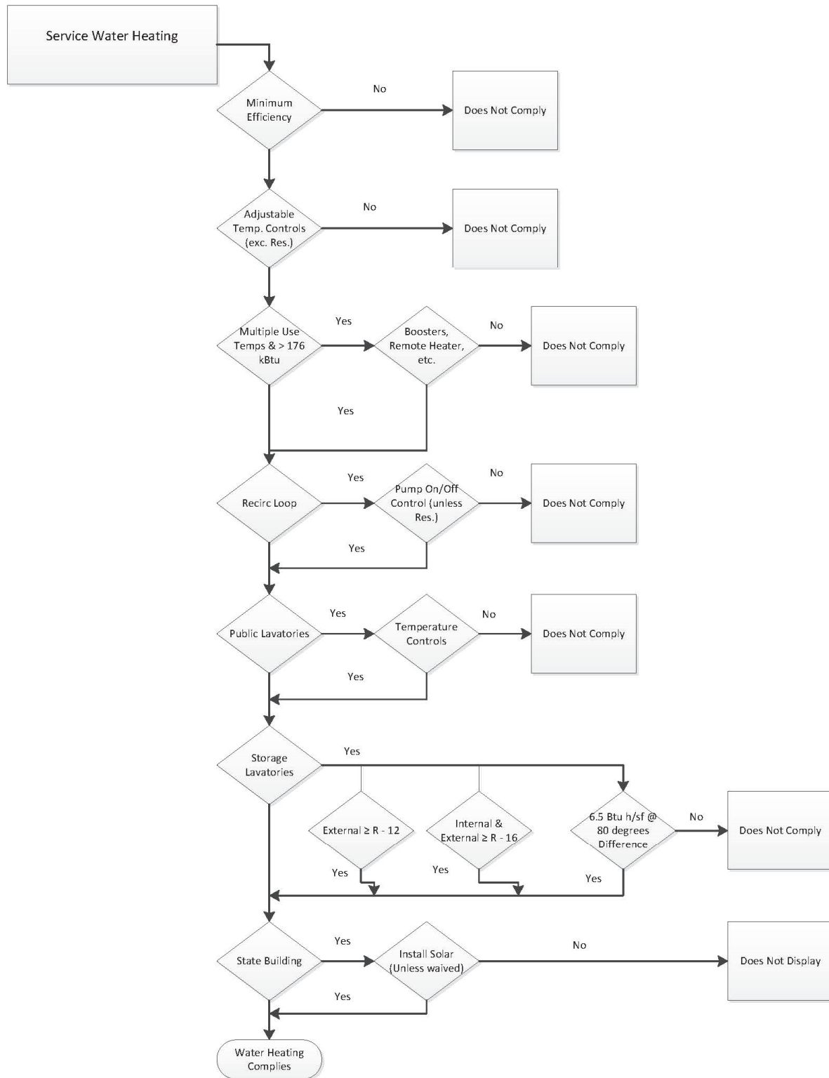
Figure 4-3132: Service Water Heating Flowchart
