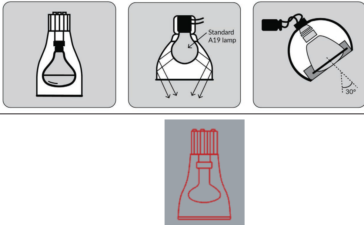
Figure 5-1: Examples of Luminaires with Line-Voltage Lamp Holders
