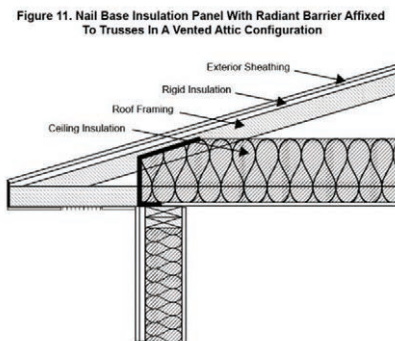
Figure 11-10. Nail Base Insulation Panel with Radiant Barrier Affixed to Trusses in A Vented Attic Configuration
