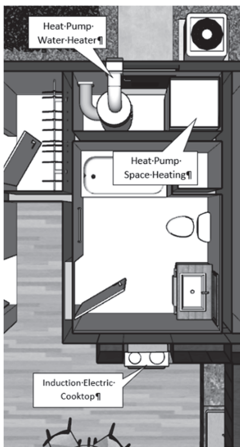
Figure 88: Garden Style Multifamily Case Study: Approved Electric Appliances Installed
