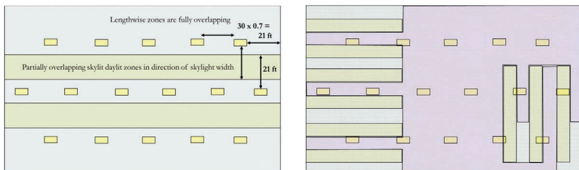
Figure 3-21: Comparison of Skylit Area for Calculating Minimum Skylit Area and the Skylit Daylit Zone for Controlling Luminaires in §130.1(d)
