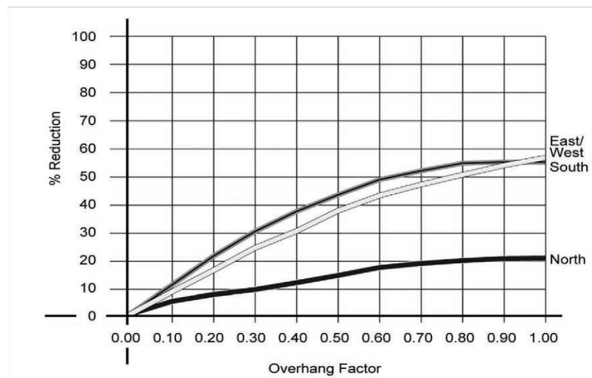
Figure 3-15: Graph of Overhang Shading Factors
