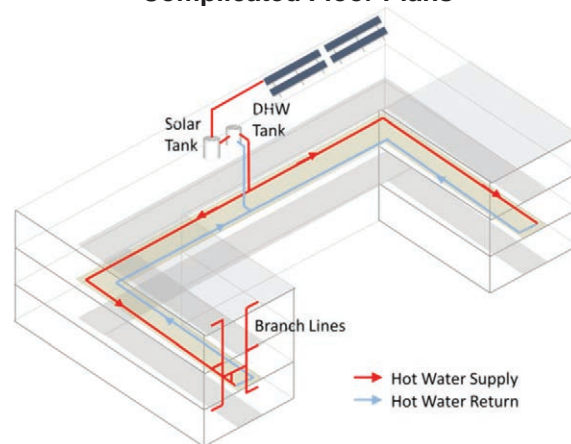
Figure 4-3435: Examples of Dual-Loop Recirculation System Designs in Buildings That Have Complicated Floor Plans
