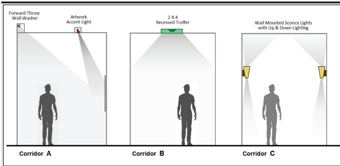
Figure 5-22 Corridors with Accent Lighting and General Lighting: A Corridor with wall washer and accent luminaires (left image); a Corridor with Recessed Troffer Luminaires (center image); a Corridor with Scone Luminaires (right image)
