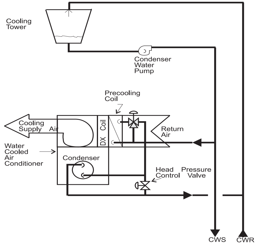
Figure 4-4041: Air-Precooling Water Economizer
