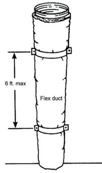
Figure 11-43: Minimum Spacing for Supporting Vertical Flex Ducts
