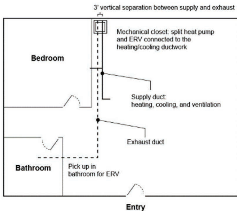
Figure 11-29: Example of Balanced Ventilation with Heat Recovery: Unitary ERV
