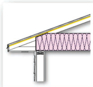
Figure 14: NFRC Label, NFRC Door Label, and R-21 Framed Wall and R-30 Attic Roof Details
