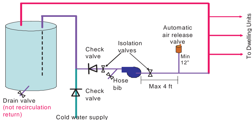
Figure 4-3233: Backflow Prevention
