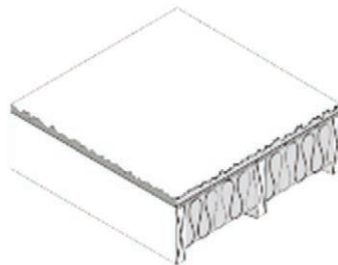
Figure 25: 4th: Raised Floor (2022 Ref. App. Fig. 4.4.2)
