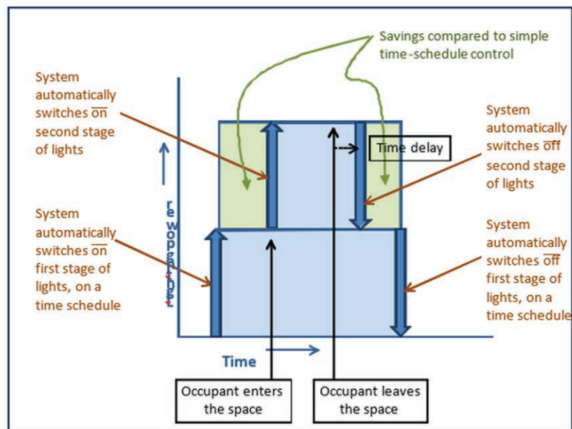
Figure 5-8 Functional Diagram for Partial-OFF Occupant Sensor
