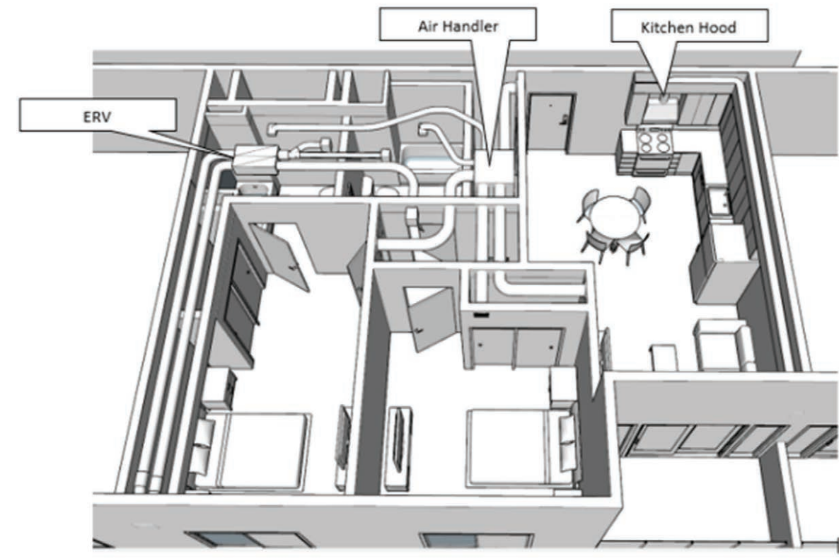
Figure 63: Mid-Rise Multifamily: 5th Floor Apartment HVAC Supply, ERV and Kitchen Hood Layout with Ducts
