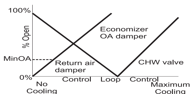
Figure 4-2627: Typical Air-Side Economizer Control Sequencing
