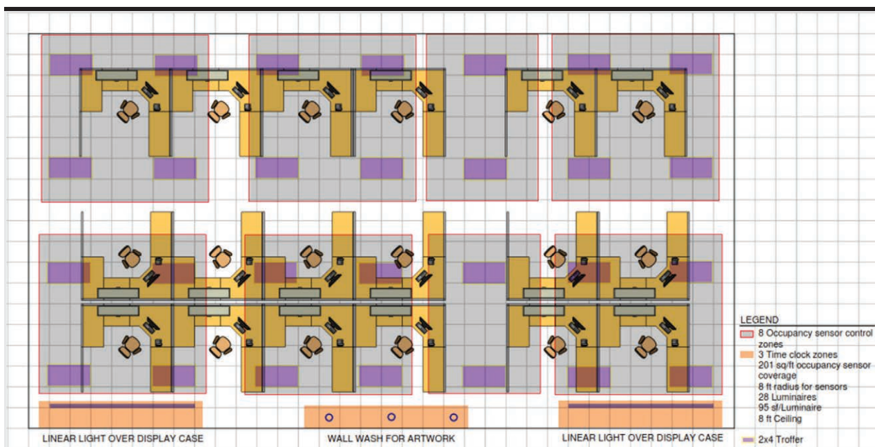
Figure 5-9 (for Example 5-5) An Office Plan with Occupant Sensing Control Zone Layout
