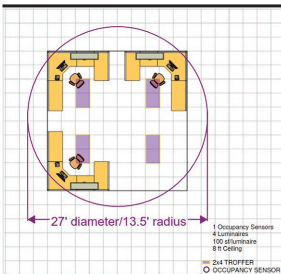
Figure 5-13 (for Example 5-9) An Office Plan with Occupant Sensing Control Zone Layout
