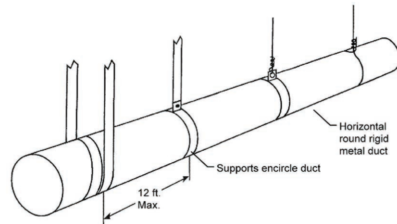
Figure 11-40: Options for Suspending Rigid Round Metal Ducts
