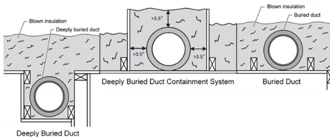
Figure 11-53: Buried Ducts on Ceiling and Deeply Buried Ducts
