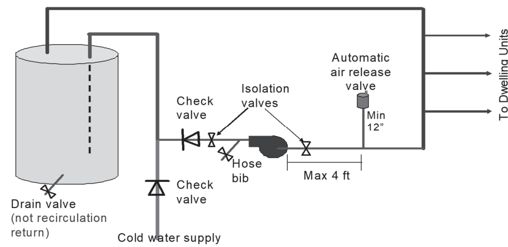
Figure 11-77: Mandatory Central Recirculation System Installation Requirements
