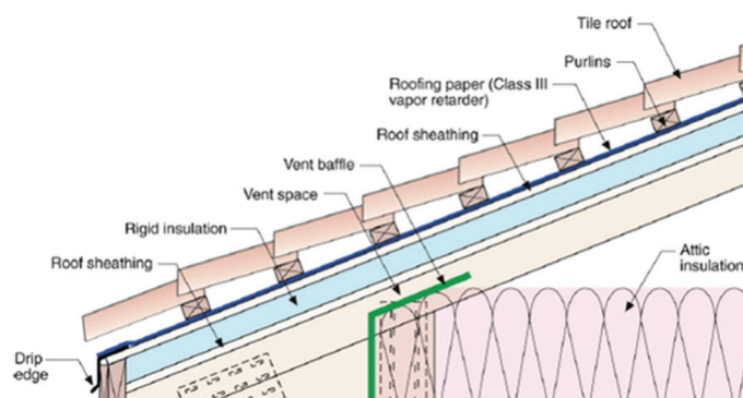
Figure 3-39: Battens (Purlins) Installed W with Above-Roof Deck Insulation
