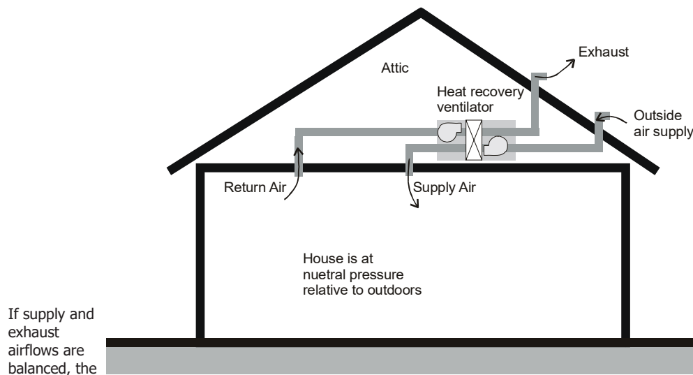
Figure 4-31: Balanced Ventilation Example 1 – HRV or ERV
