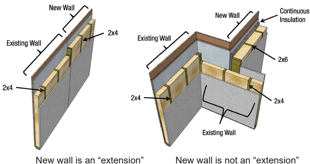
Figure 9-1: Wall Extension
