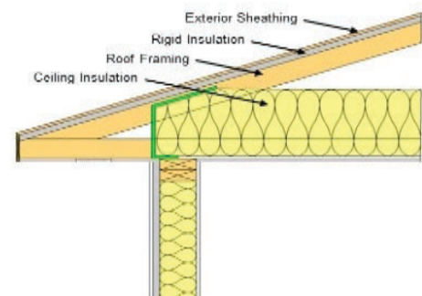
Figure 3-45: Nail Base Insulation Panel W with Radiant Barrier Affixed to Trusses in a Vented Attic Configuration
