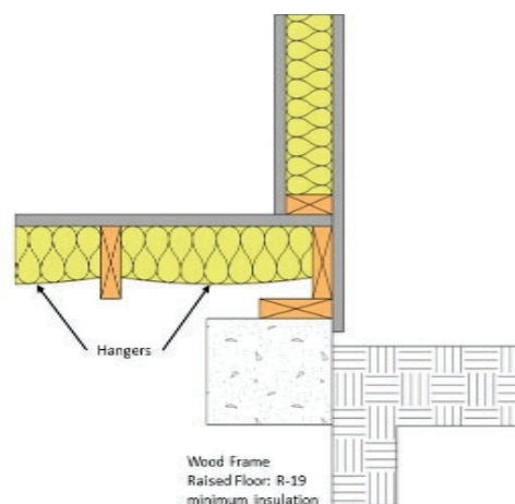
Figure 3-30: Raised Floor Insulation
