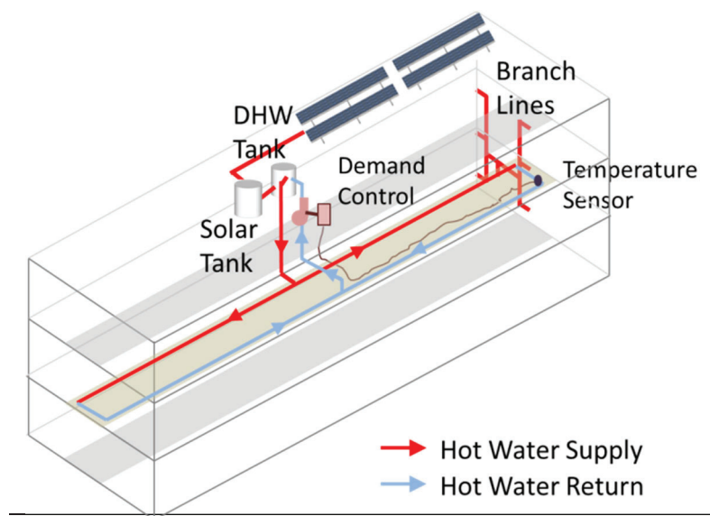
Figure 5-15: Standard Multifamily Central Distribution System
