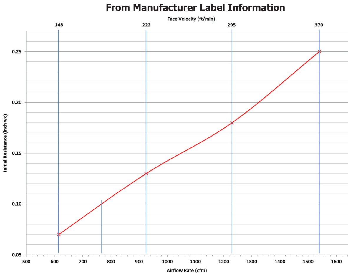
Figure 4-6. Plot of Pressure drop vs. Airflow for a 20" X 30" X 1" Depth Air Filter
