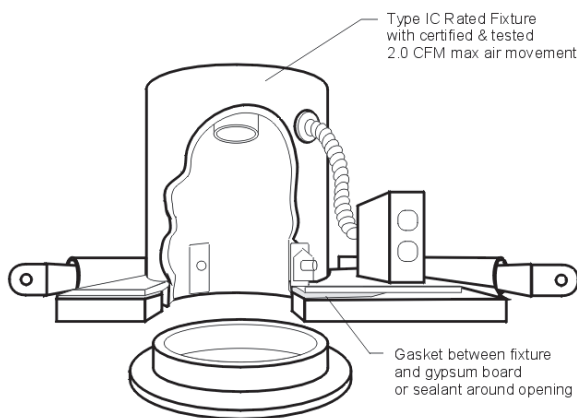
Figure 3-21: IC-Rated Luminaire (Light Fixture)
