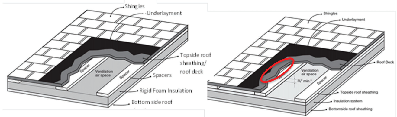
Figure 3-40: Above-Roof Deck Insulation and Air Spacers Installed W with and W without A Second Layer of Roof Top Sheathing
