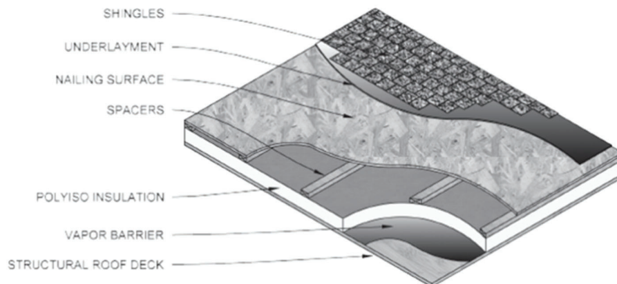
Figure 3-41: Asphalt Shingles and Spacers Installed W with Above-Roof Deck Insulation
