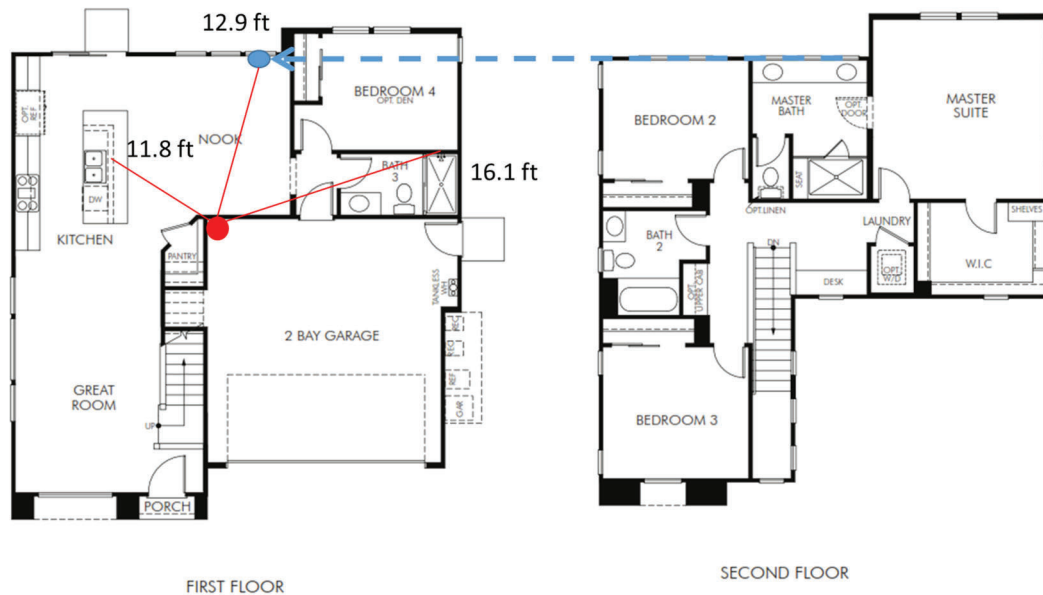
Figure 5-14: Weighted Distance Calculation for the 1,814 Plan with a Centrally Located Water Heater
