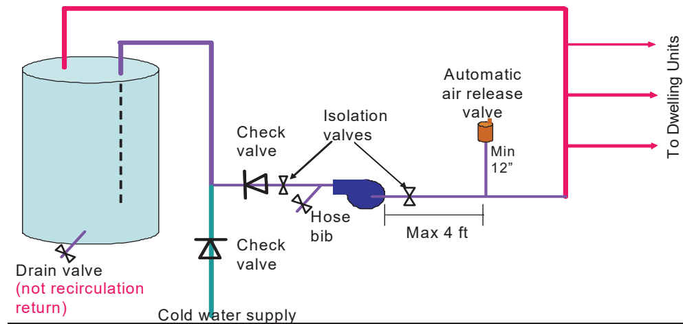
Figure 5-6: Mandatory Central Recirculation System Installation Requirements
