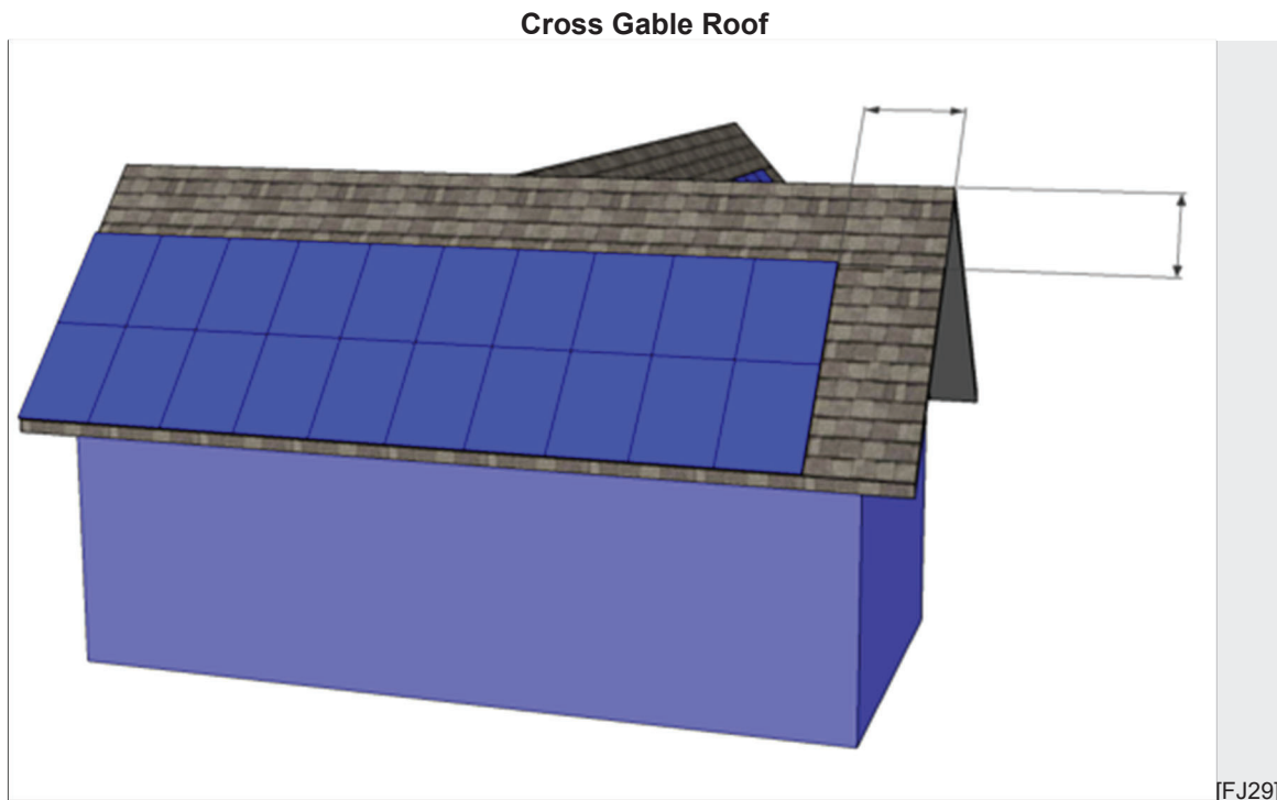
Figure 7-6: The Following Illustrations Demonstrate Some Acceptable Solar Access Techniques.
