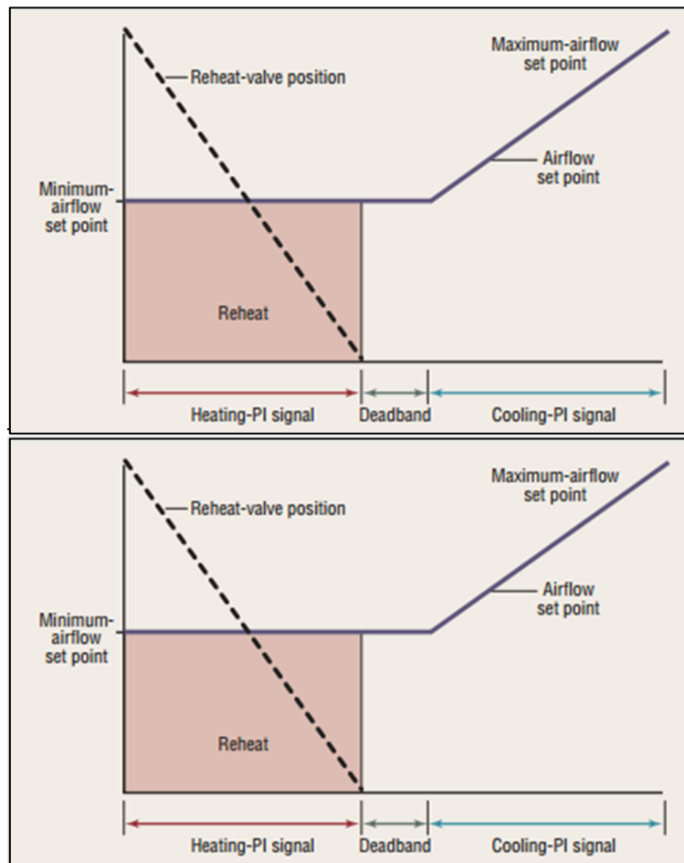
Figure 9: Single Maximum VAV Box Control
