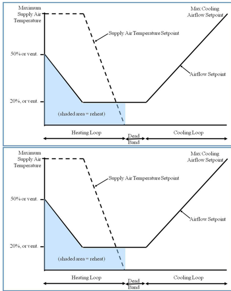
Figure 10: Dual Maximum Control Sequence
