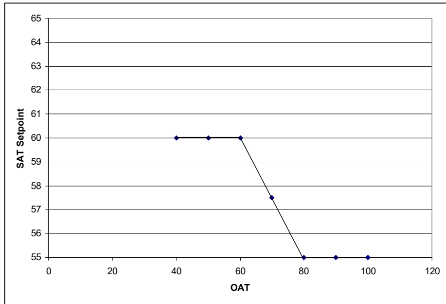
Figure 11: SAT Cooling Setpoint Reset Based on Outdoor Air Temperature (OAT)
