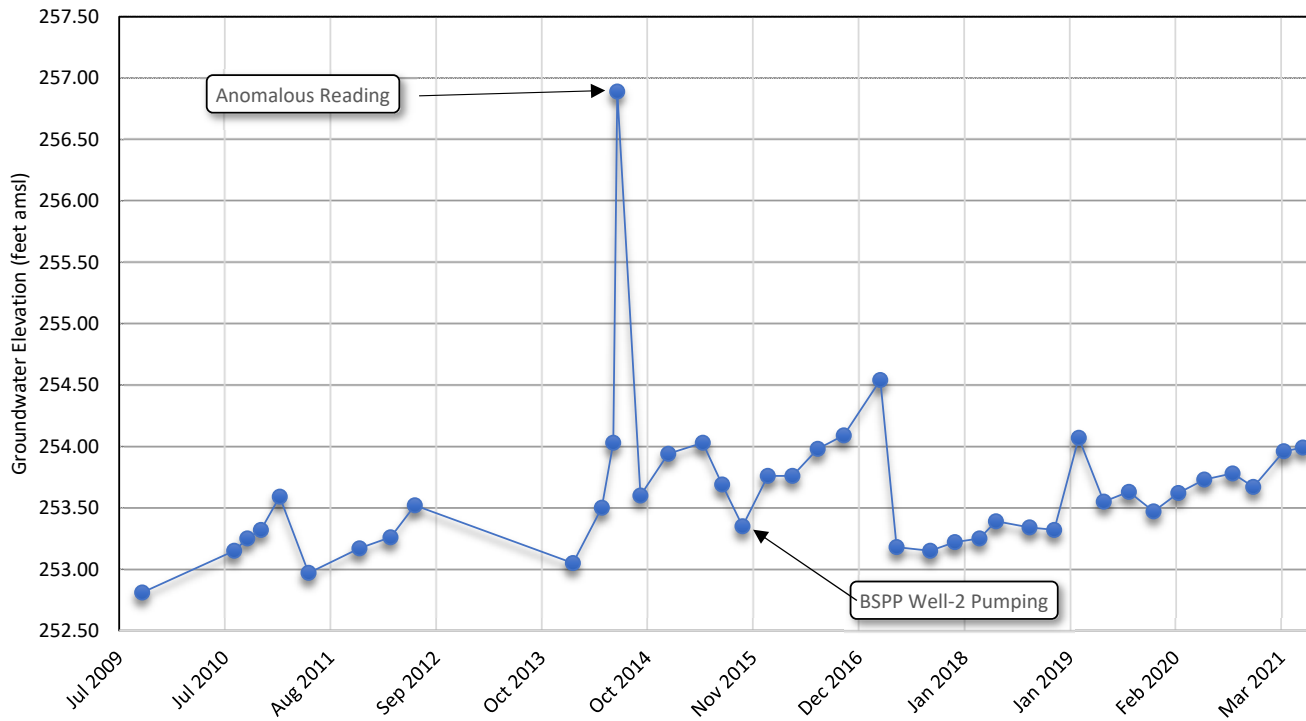
Chart 2 BSPP WO-2 Hydrograph
