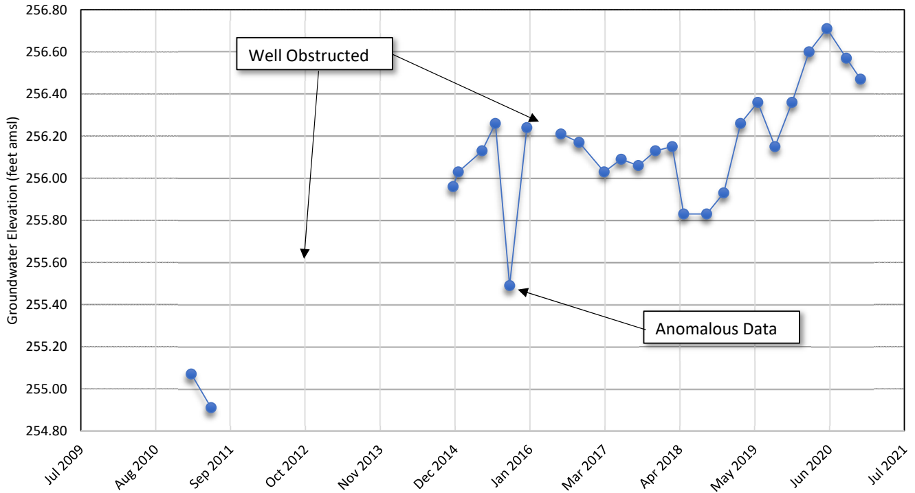
Chart 8 County Well 36G1S Hydrograph
