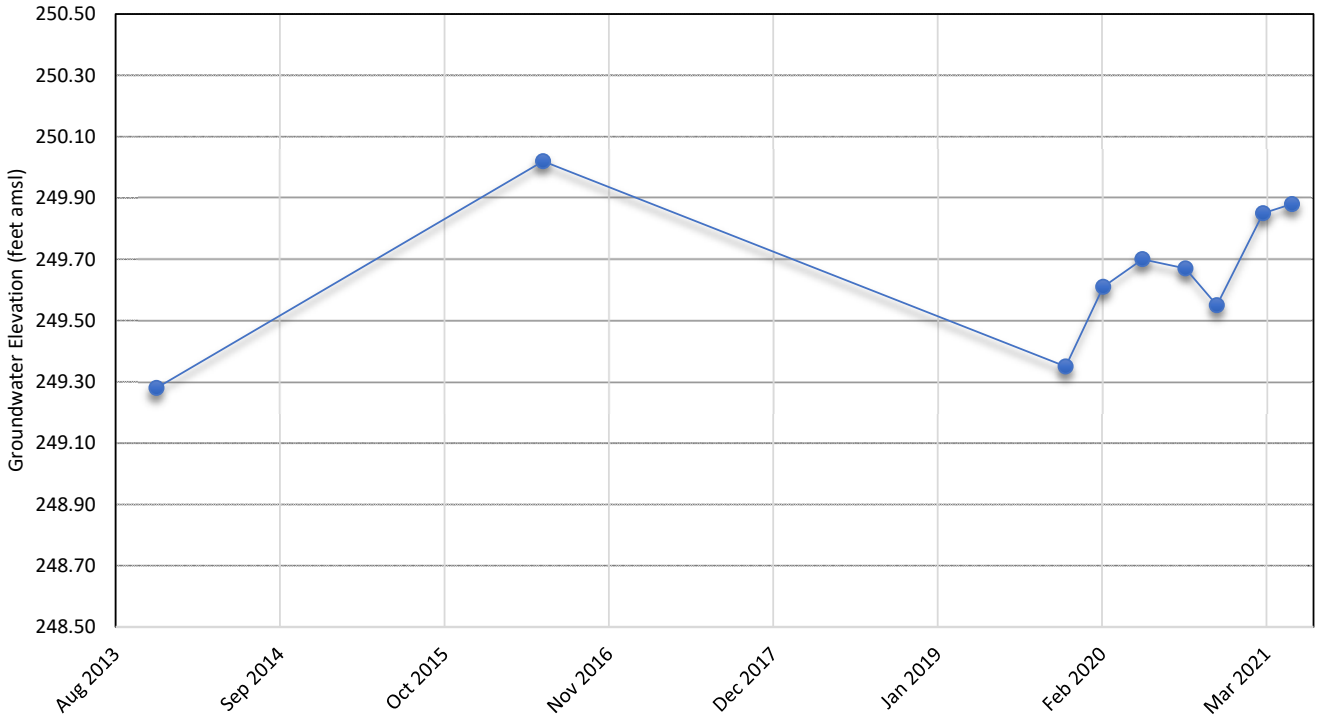
Chart 11 6S/22E-19N2S Well Hydrograph
