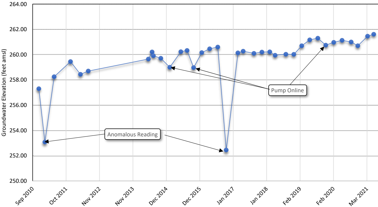
Chart 4 Gila Farm Well Hydrograph
