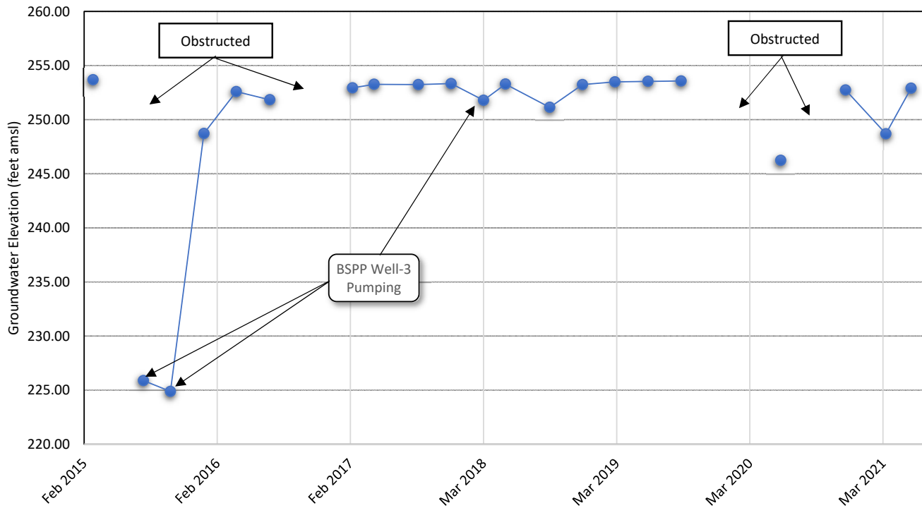
Chart 3 BSPP Well-3 Hydrograph
