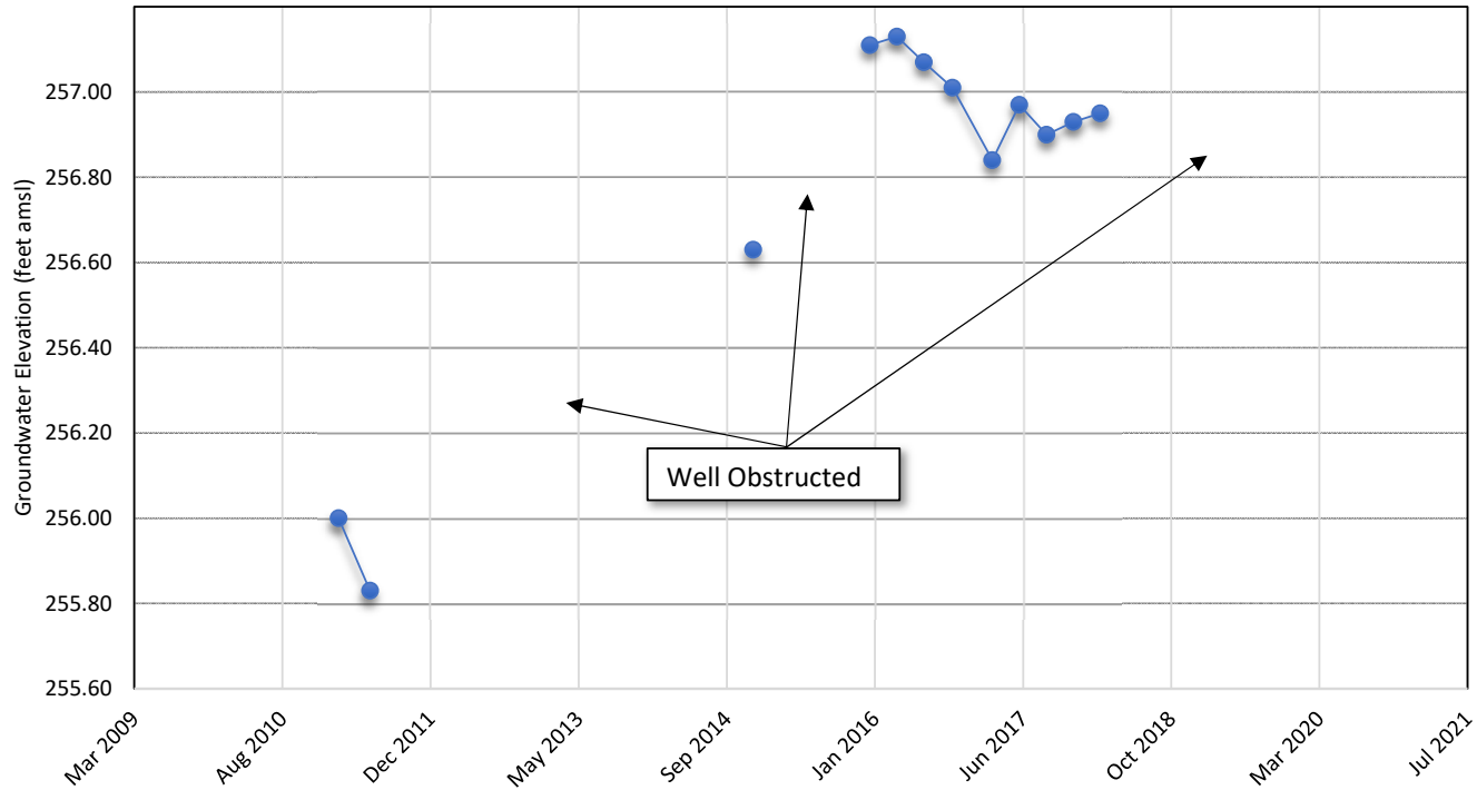
Chart 6 County Well 25L1S Hydrograph
