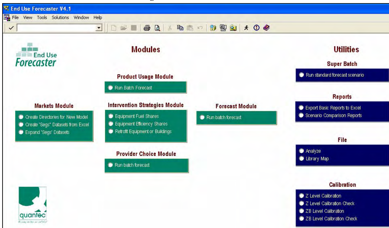
Figure 3. Main Dashboard
