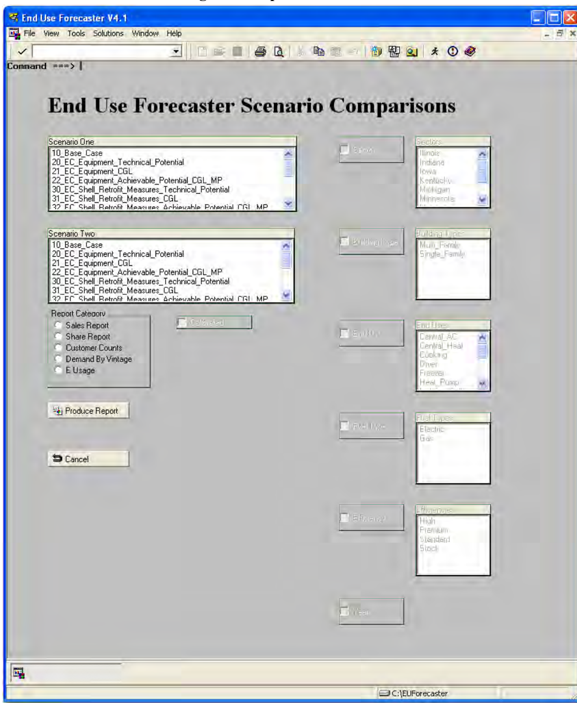
Figure 4. Report Customization
