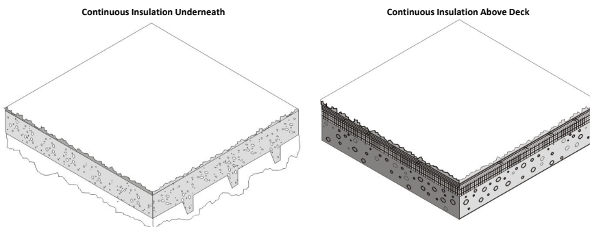
Figure 4.4.6 – Concrete Raised Floors
