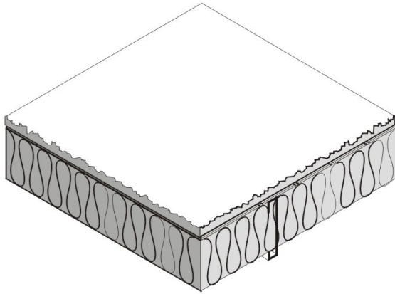
Figure 4.4.5 – Metal Framed Floors without a Crawl Space
