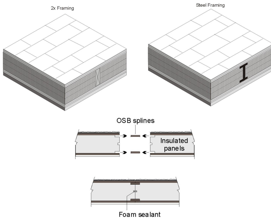
Figure 4.2.3 – SIPS Roof/Ceiling
