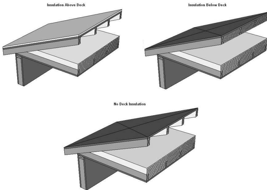
Figure 4.2.1 – Wood Framed Attic Roofs
