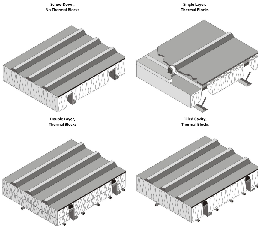
Figure 4.2.7 – Metal Building Roofs
