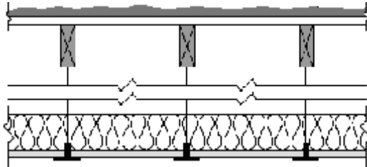
Figure 4.2.8 – Insulated Ceiling with Removable Panels
