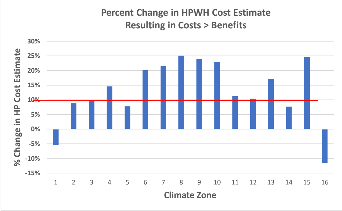
Figure 2. Scenario with Equal Maintenance Cost for Gas Instantaneous and HPWH
