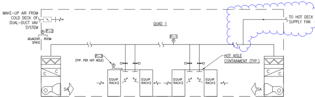
Figure 6. Computer room heat recovery example mechanical diagram: DFDD.
