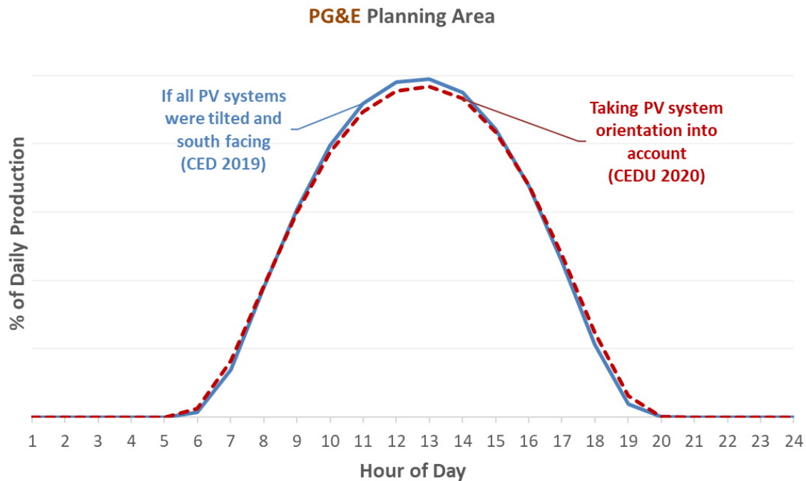
Figure 6: PV Production for a Day in Early July
