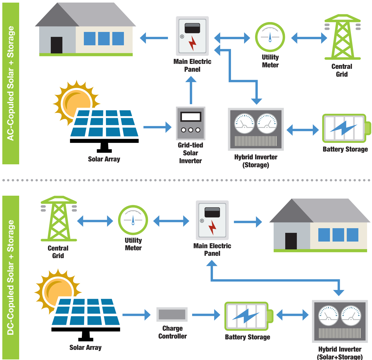
Q5 FIGURE 1: AC- and DC-coupled solar+storage
