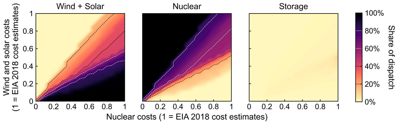
Fig. A4. Least-cost shares of dispatched generation for Case #4 (wind + solar + flexible nuclear generation + energy storage) as a function of costs of nuclear power (horizontal axis) and wind and solar electricity (vertical axis).
