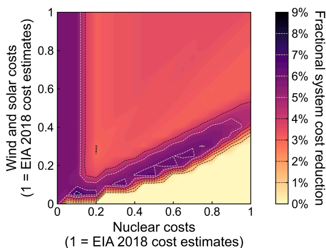
Fig. A13. Fractional difference in system cost as a function of costs of nuclear power (horizontal axis) and wind and solar electricity (vertical axis) for least-cost systems with wind, solar, constant or flexible nuclear generation, and energy storage (Case #3 and Case #4).
