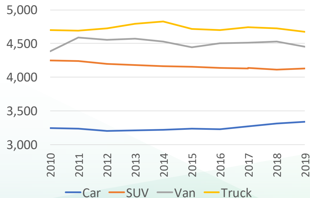
Average vehicle curb weight by vehicle class (pounds)
