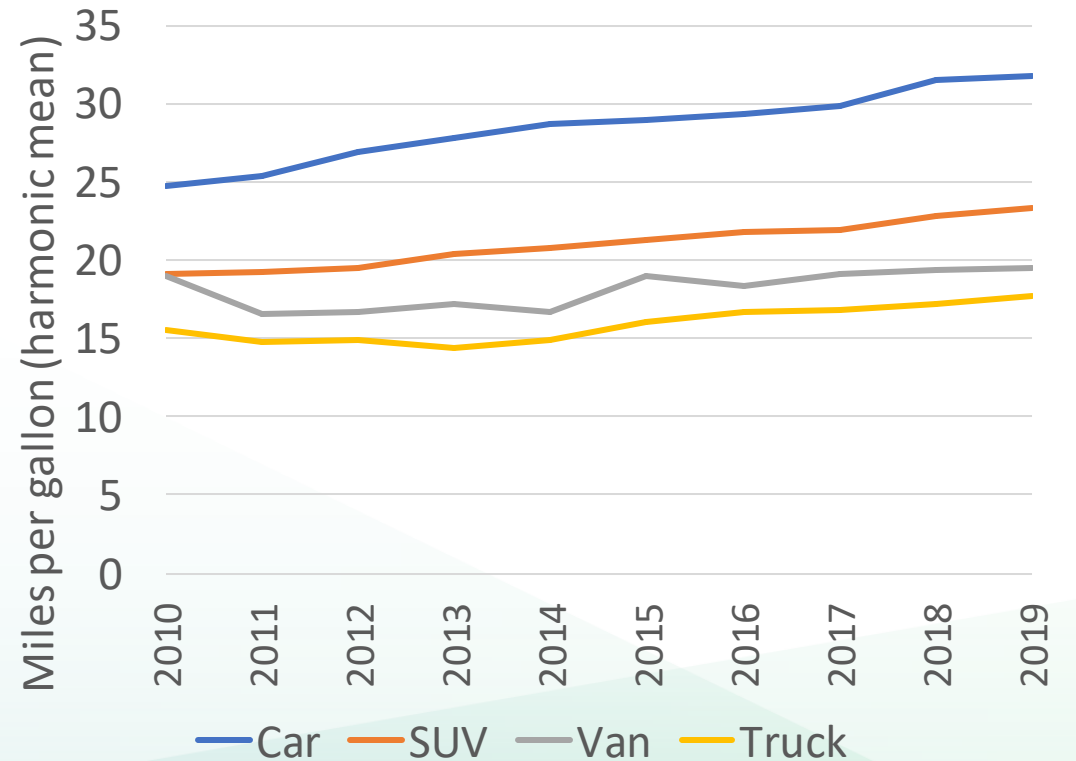
Fuel efficiency by vehicle type
