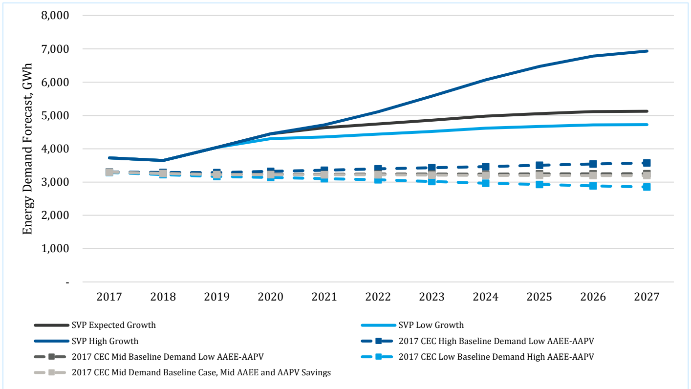
Figure 4-2 Energy Requirements Comparison: SVP Forecast vs. CEC Forecast for SVP
