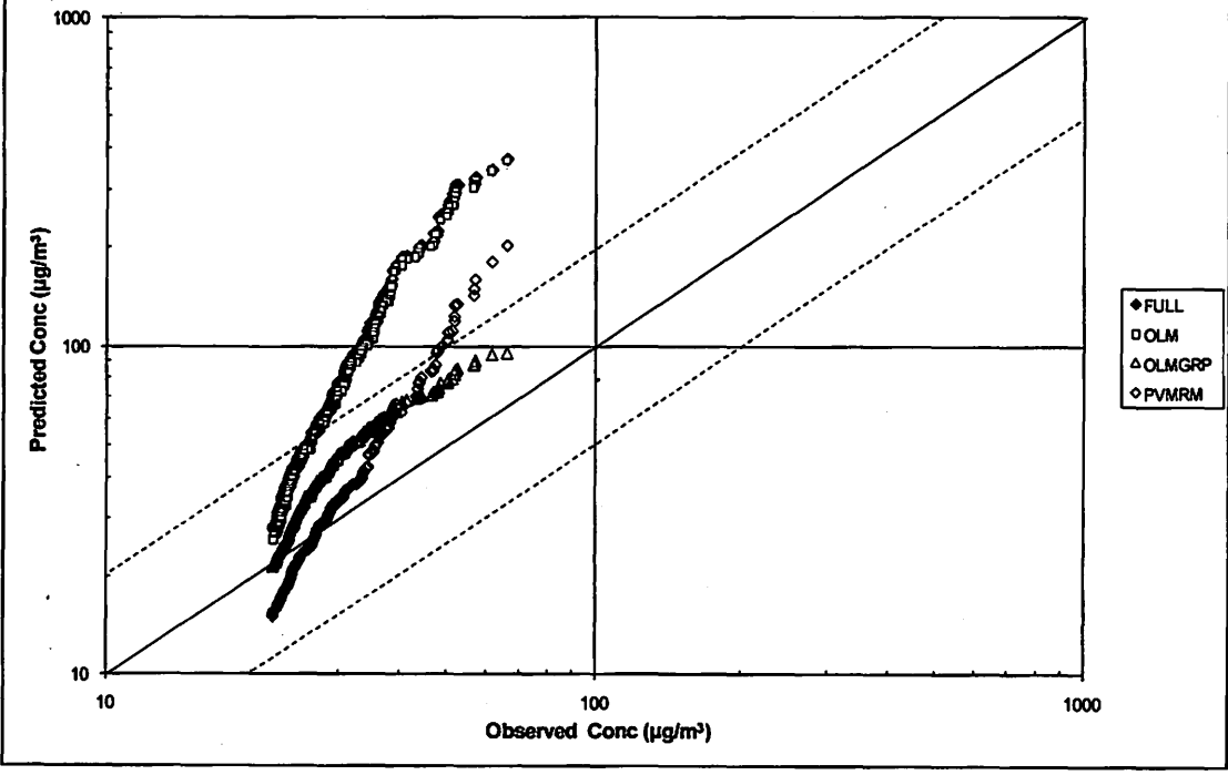
Figure A-2. AERMOD Model Evaluation - New Mexico South Monitor - Hourly NO2 Q-Q Plot
