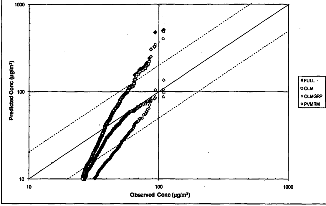
Figure A-1. AERMOD Model Evaluation - New Mexico North Monitor - Hourly NO2 Q-Q Plot
