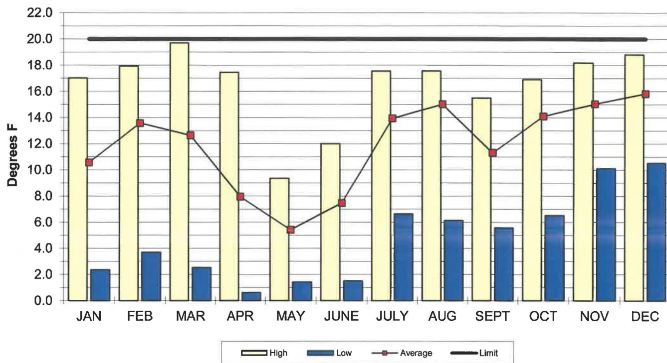
DAILY AVERAGE DELTA T (Only Units 1 & 2 Operating)
