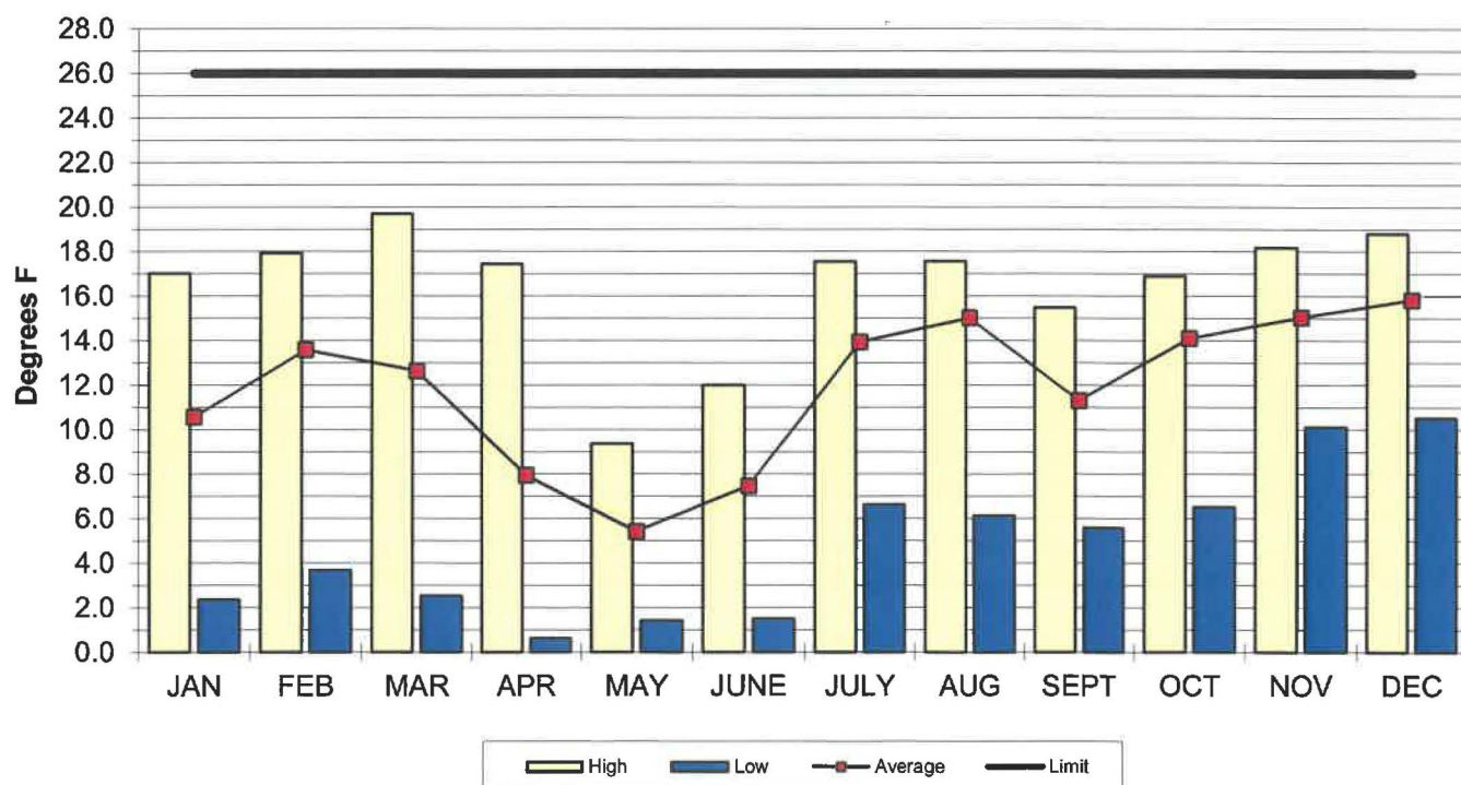
INSTANTANEOUS MAXIMUM DELTA T (Only Units 1 & 2 Operating)
