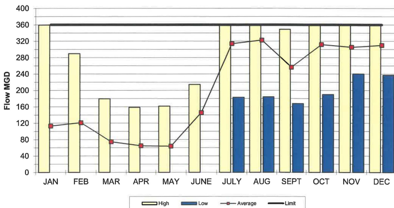
EFFLUENT 002 Once Through Cooling for Units 1 & 2 Only
