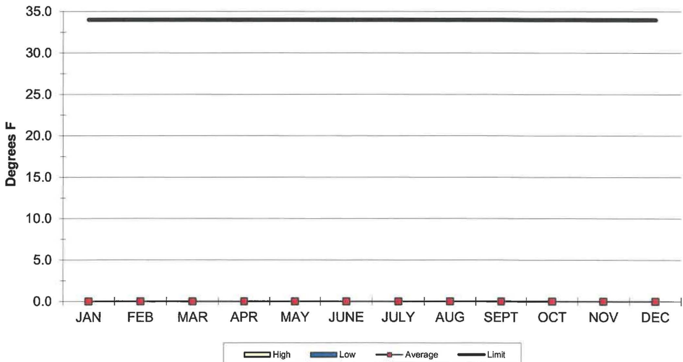
INSTANTANEOUS MAXIMUM DELTA T (Only Units 6 & 7 Operating)
