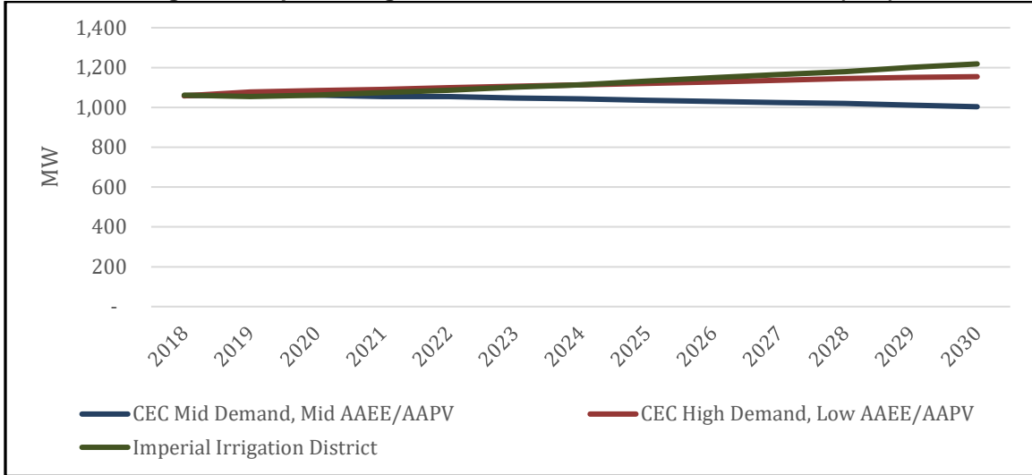
Figure 2: Imperial Irrigation District and CEC Peak Forecasts (MW)
