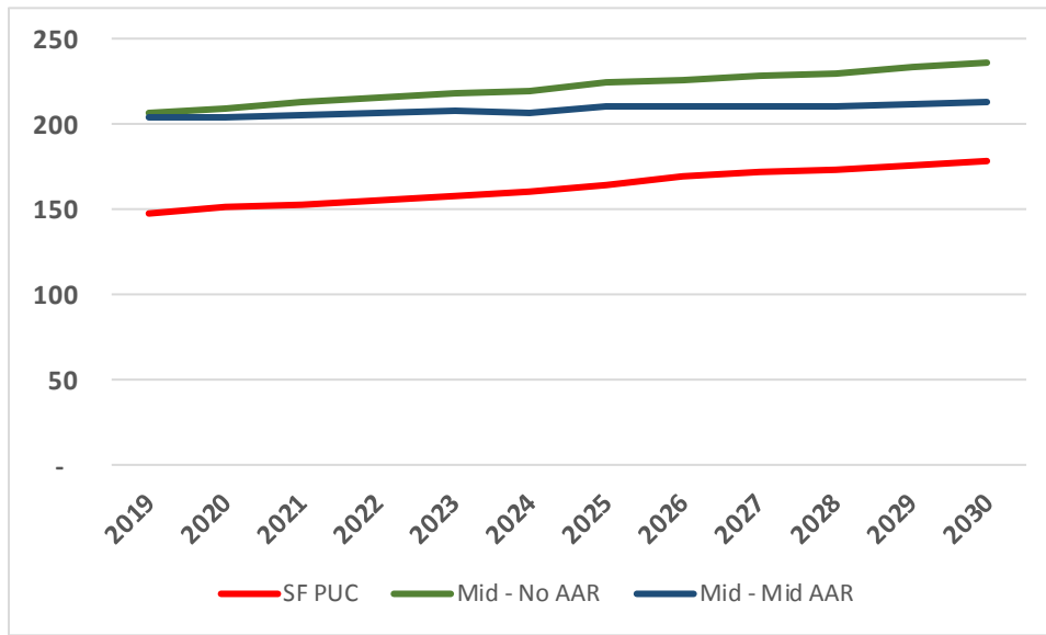
Figure 2: SFPUC and Energy Commission Peak Forecasts 2019-2030 (GWh)
