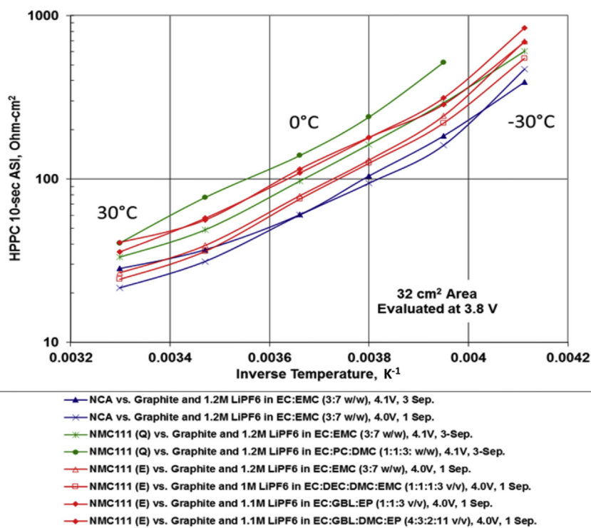
Fig. 5. Area specific impedance (ASI) vs. inverse temperature for a typical lithium-ion battery [62,63].
