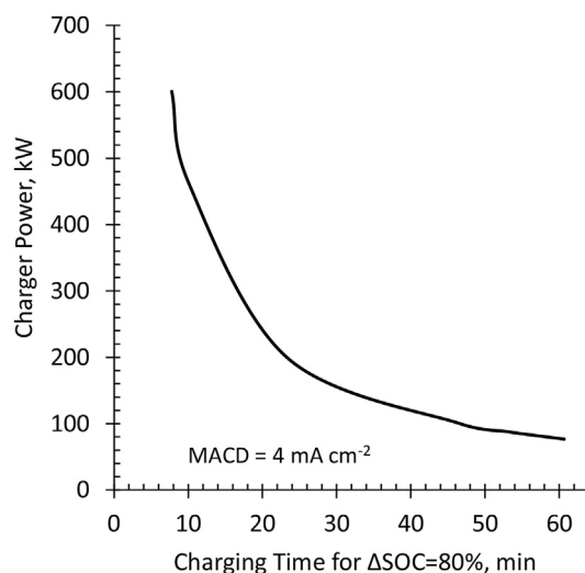
Fig. 7. Charger power needed to recharge a 85 kWh, 300 kW, 900 V battery pack to raise its SOC by 80% (from 15% to 95%) within a specified charging time.
