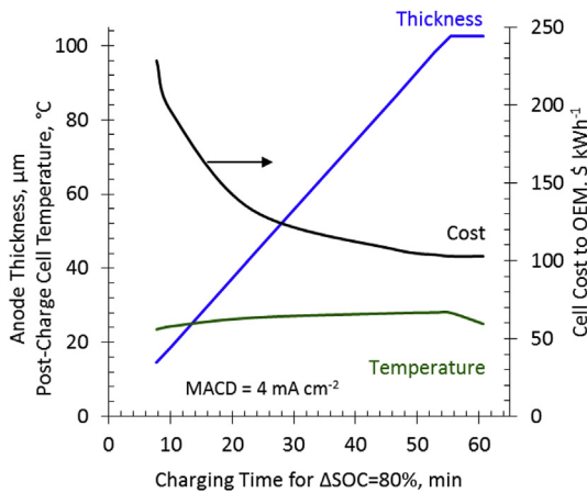
Fig. 8. Effect of charging time on the required anode thickness, the post-charge cell temperature charge, and the cell cost. Assumptions: No pack cooling, maximum allowable current density to avoid lithium plating (MACD) = 4 \text{ mA cm}^{-2} , anode/cathode thickness ratio = 1.12, NMC622-Graphite, 85 kWh pack.
