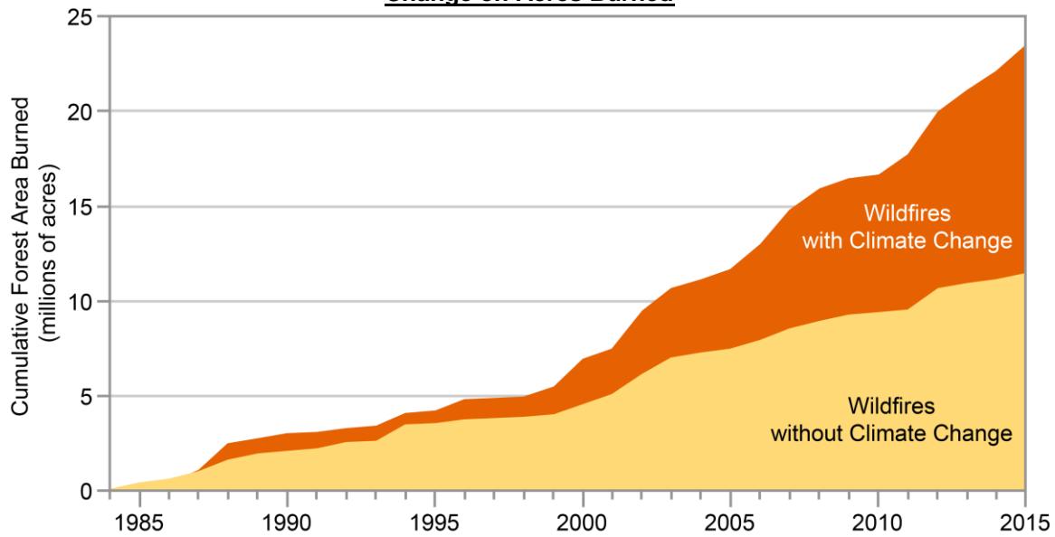
Figure 28: Wildfire in the Western United States (1984–2015): Estimated Impact of Climate Change on Acres Burned
