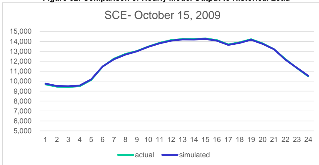
Figure 62: Comparison of Hourly Model Output to Historical Load
