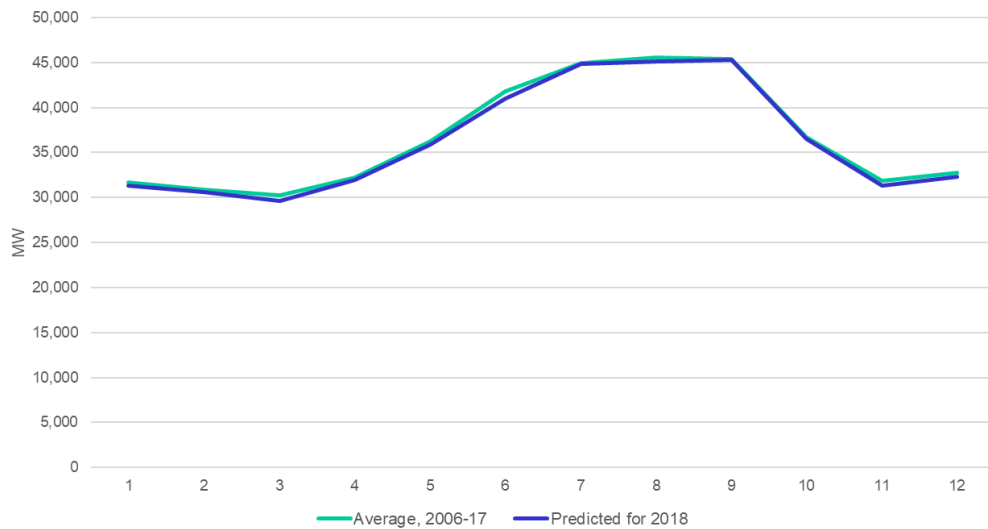
Figure 63: Comparison of Monthly Peaks—California ISO History vs. Hourly Models
