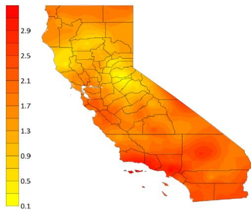
Figure 25: Historical Changes in Annual California Temperatures: 1901-1960 vs. 1986-2016
