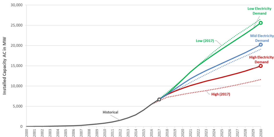
Figure 60: Statewide Behind-the-Meter PV Capacity
