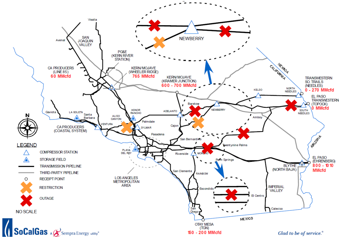
Figure ES-6: Southern California Gas System Outages (as of April 2018)
