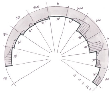
(b) Within each compass sector, the highest altitude angle is selected and used for that entire sector. This datum is shown for a single point of reference on the array.
