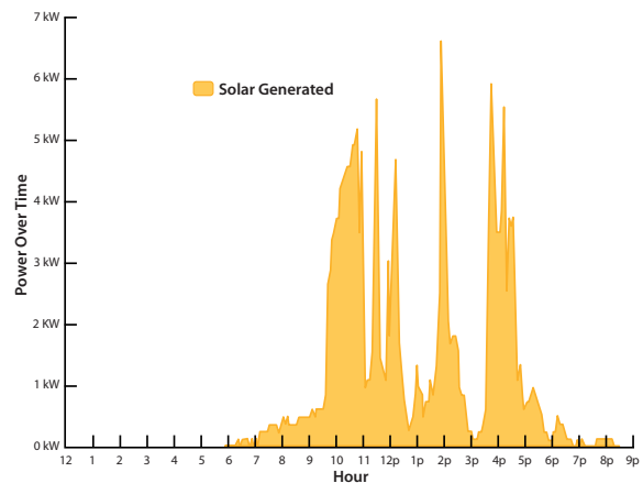
Figure 1. The Variable Generation of a Single Solar PV System. In most cases, the variability of a single system is balanced out by other systems in the vicinity.
