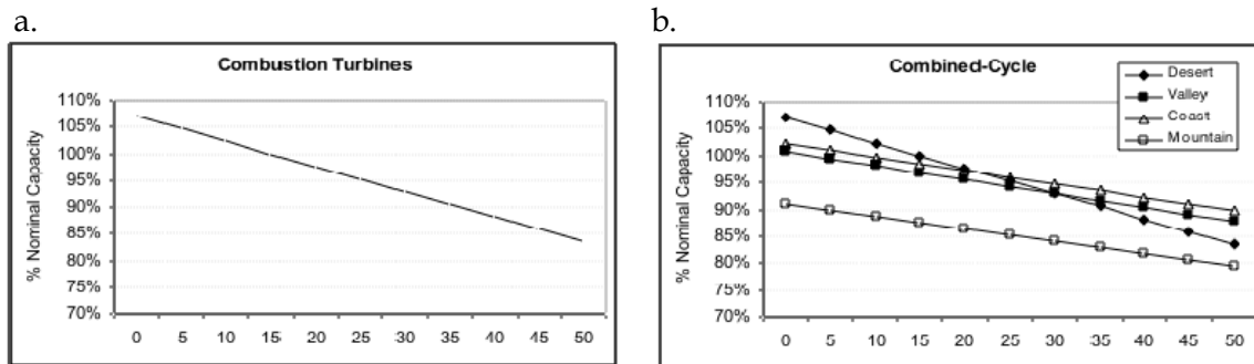
Figure 3. Change in Turbine Capacity as a Function of Ambient Temperature
