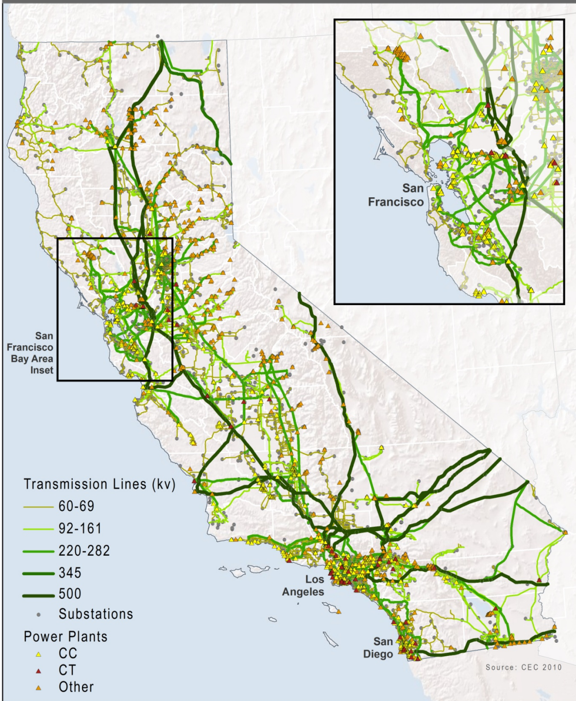
Electrical Power Infrastructure Examined in this Study
