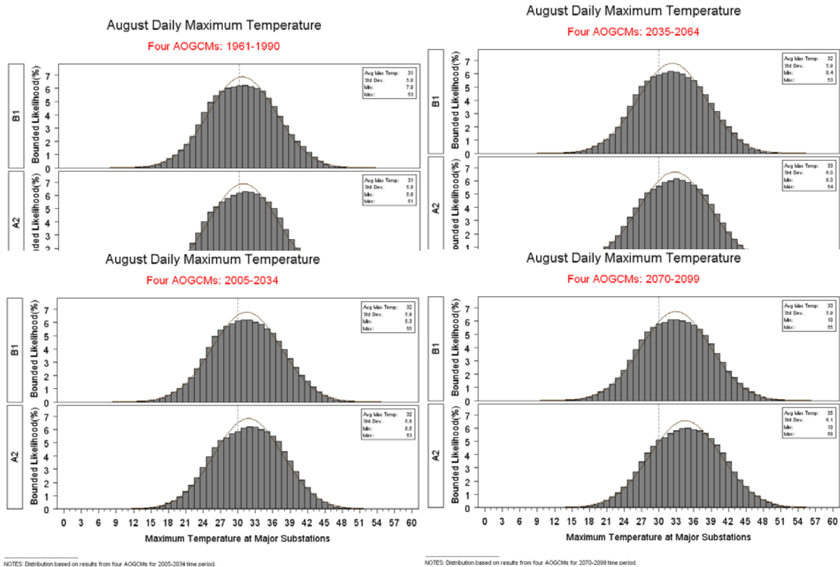
Figure B-2. Projected Range of August Daily Maximum Temperatures at California's Major Substations
