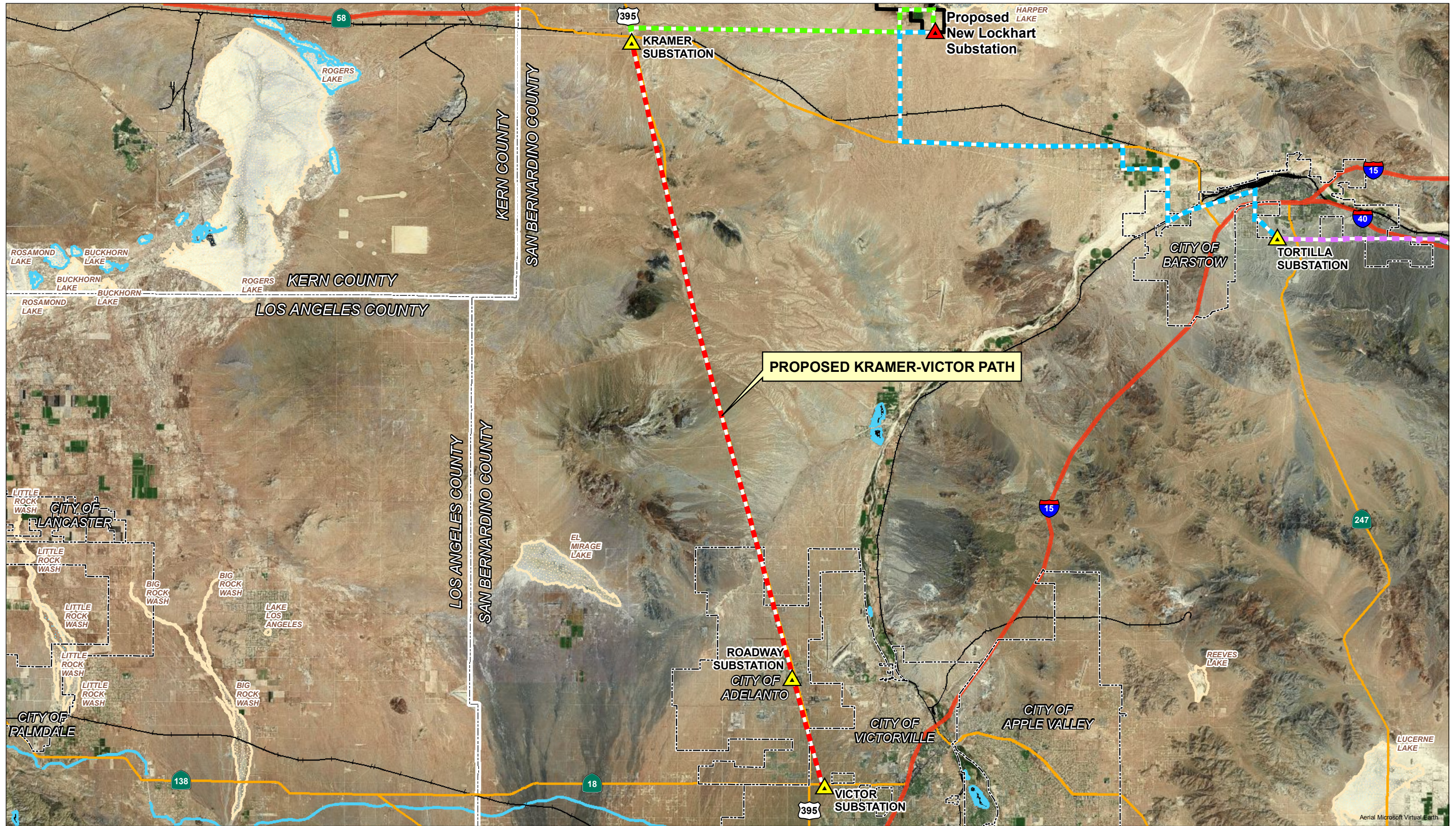
FIGURE 3-6 PROPOSED NEW TELECOMMUNICATION FIBER OPTIC CABLE CONNECTING KRAMER SUBSTATION TO VICTOR SUBSTATION
